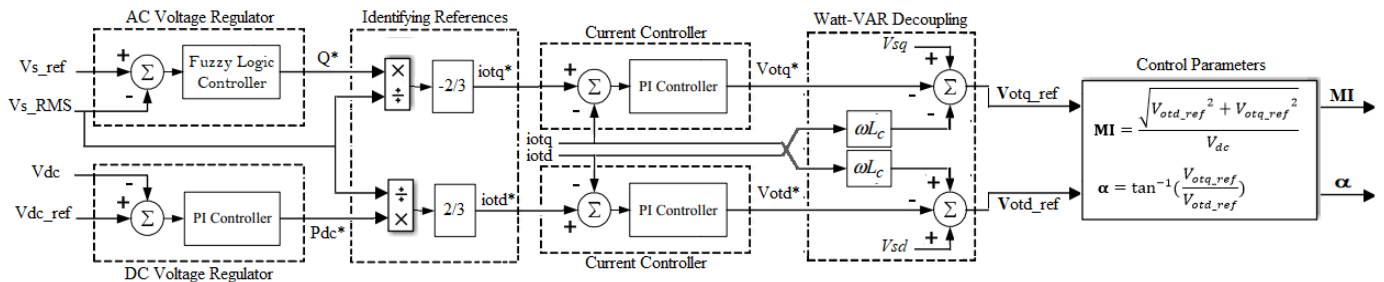
Figure 4. Control Scheme.
