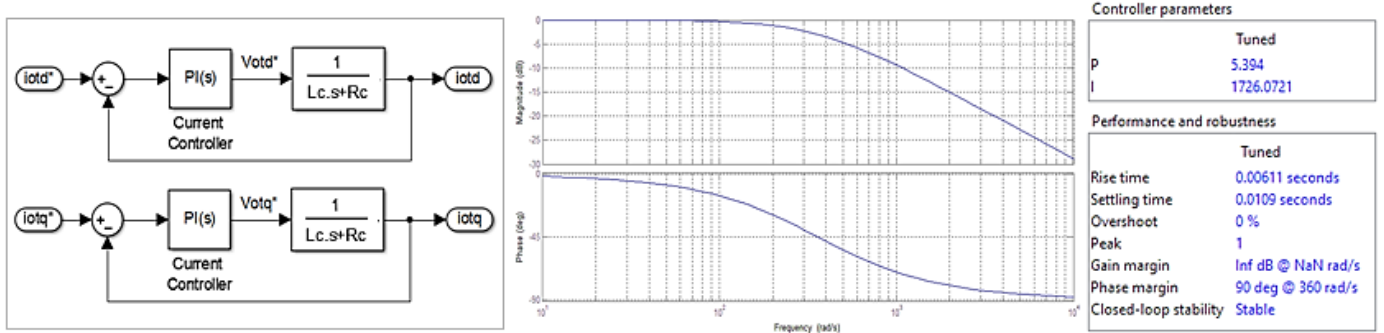
Figure 5. Current loops frequency response with controller parameters and performance.
