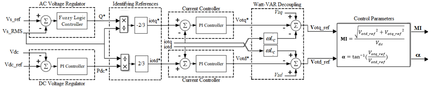
Figure 4. Control Scheme.
