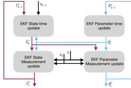
Fig. 4. DEKF Structure
