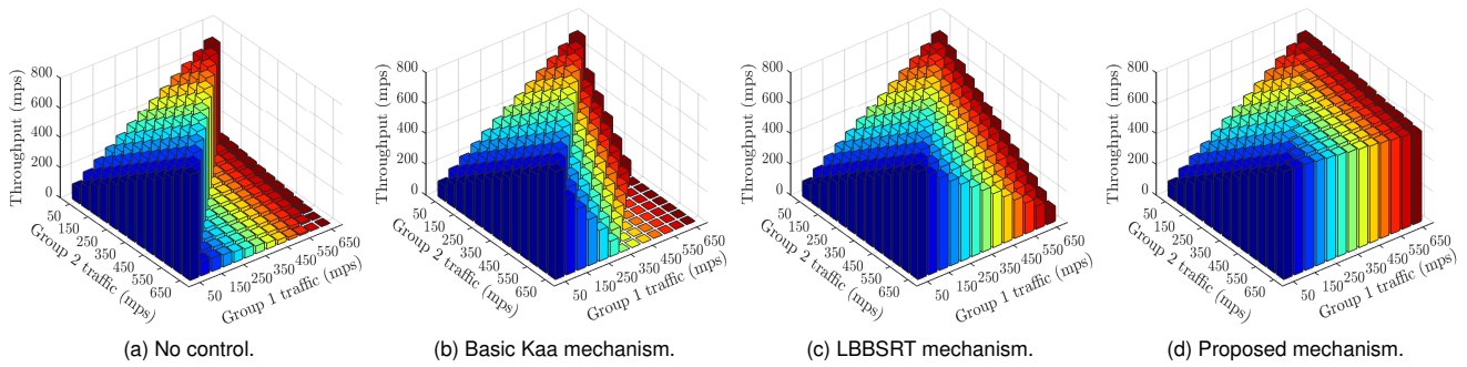
Figure 14. Servers' throughput by increasing traffic
