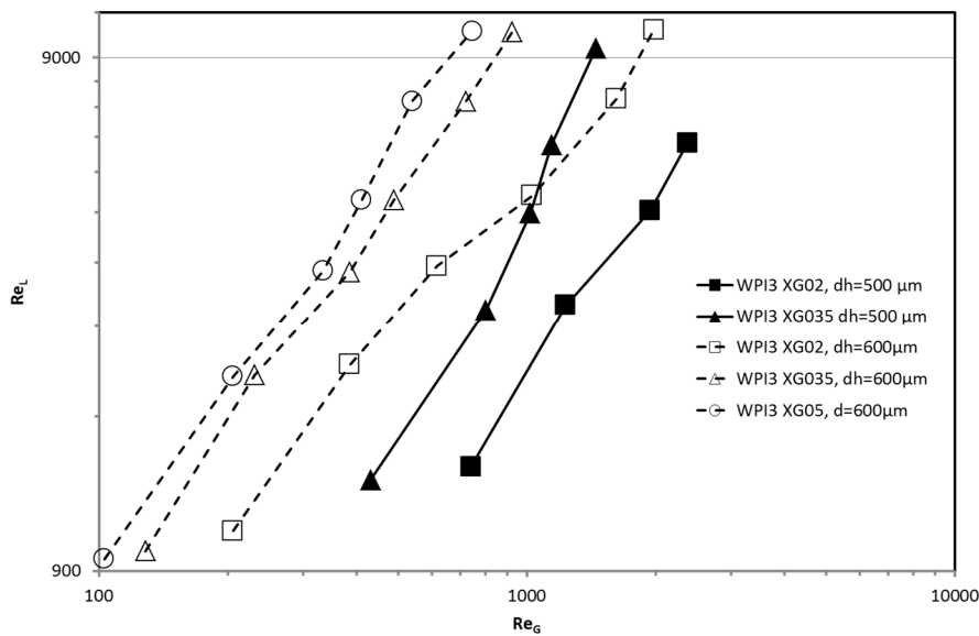
Fig. 7: Comparison of the limit between dispersed flow regime and churn or plug flow regime observed
