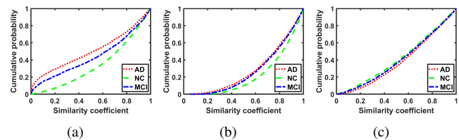
Fig. 2. Statistics of the similarity coefficients between subjects for a certain ROI. (a) ROI: Angular_L. (b) ROI: Hippocampus_L. (c) ROI: Cerebelum_10_R
