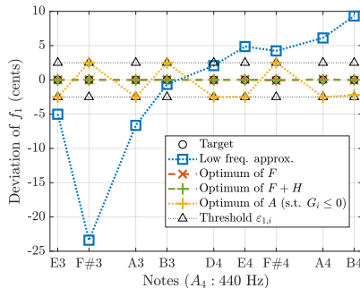
Figure 5: Deviation in cents of the first resonance frequencies from the target value for the first register (9 first fingerings). The problem with F+H is presented in Sec.5.6, the threshold \varepsilon_{1,i} and the problem “ A s.t. G_i ” are presented in Sec.5.7.
