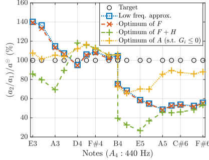
Figure 7: Ratio of magnitude of the two first frequencies resonance a_2/a_1 for each fingering, compared to the target values a^\odot .
