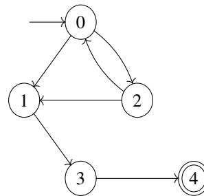
Figure 2: State machine
