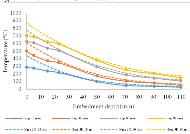
Fig. 3: Comparison between numerical and experimental temperature profiles for M12 anchors directly exposed to fire
