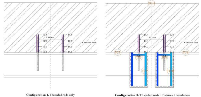
Fig. 2: Configurations of tested specimens in Al-Mansouri et al. [16]
