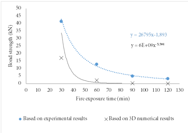
Fig. 6: Comparison between experimentally and numerically predicted bond strength vs. fire exposure time relationships for M12 anchor with insulated fixtures
