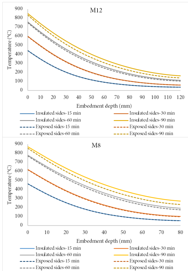
Fig. 8: Temperature profiles for M8 and M12 anchors in insulated beams and beams exposed to ambient air on all sides
