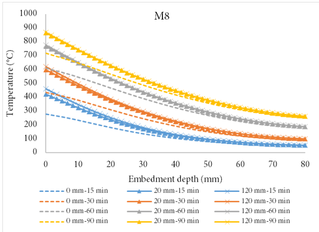
Fig. 7: Temperature profiles for M8 and M12 anchors with h_{ef}=10*d for different extended lengths
