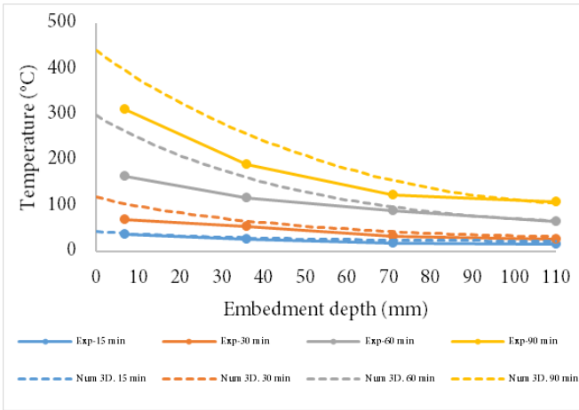
Fig. 5: Comparison between experimental and numerical temperature profiles for M12 anchor with insulated fixtures
