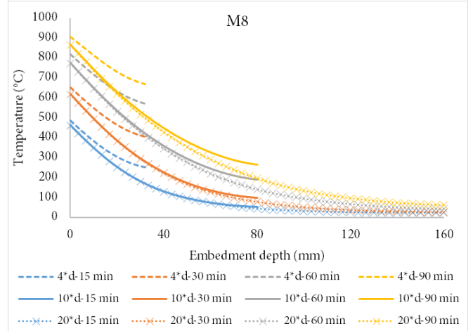
Fig. 8: Temperature profiles for M8 and M12 anchors with extended length of 10*d for different embedment depths
