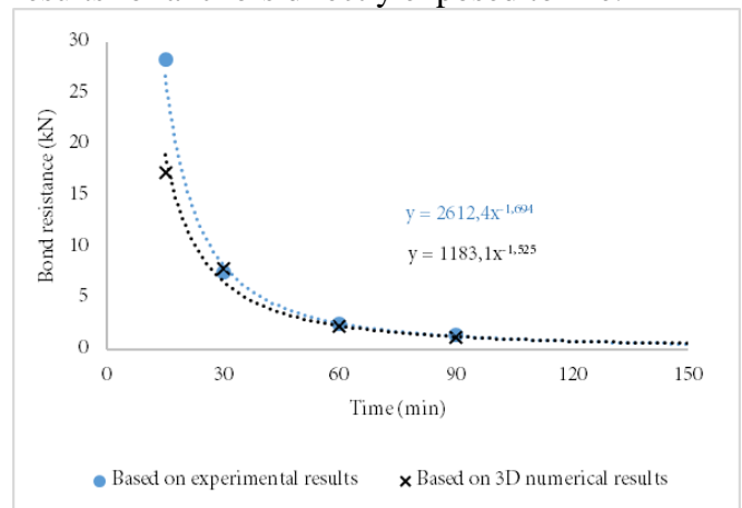
Fig. 4: Comparison between experimentally and numerically predicted bond strength vs. fire exposure time relationships for anchors directly exposed to fire
