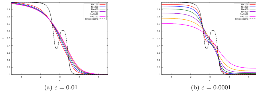
Figure 5: Water height at time t = 0.01 with the continuous initial condition for different number of cells.
