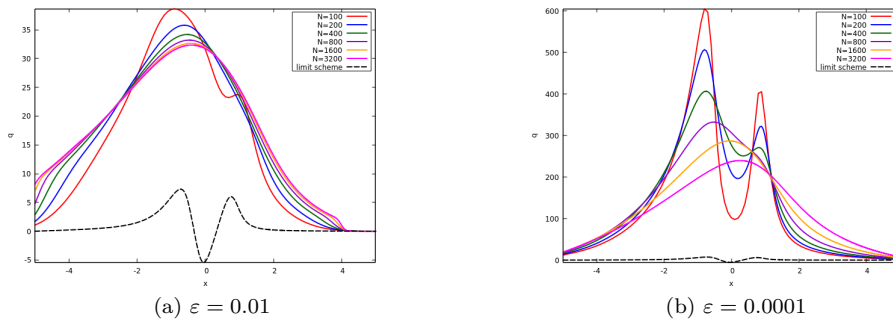
Figure 9: Order one of the water discharge at time t = 0.01 with the continuous initial condition for different number of cells.
