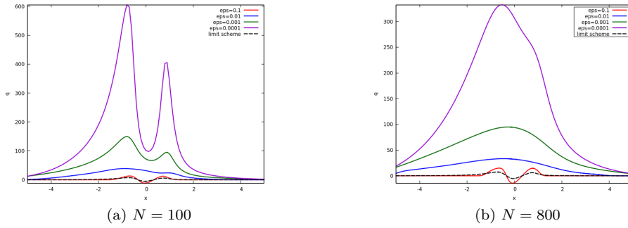
Figure 7: Order one of the water discharge at time t = 0.01 with the continuous initial condition for different values of \varepsilon .
