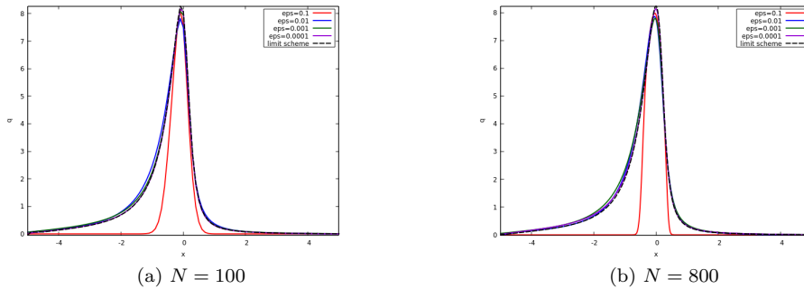
Figure 16: Order one of the water discharge at time t = 0.01 with the discontinuous initial condition for different values of \varepsilon .
