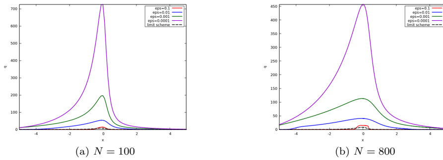
Figure 8: Order one of the water discharge at time t = 0.01 with the discontinuous initial condition for different values of \varepsilon .
