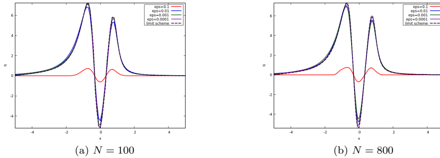
Figure 15: Order one of the water discharge at time t = 0.01 with the continuous initial condition for different values of \varepsilon .
