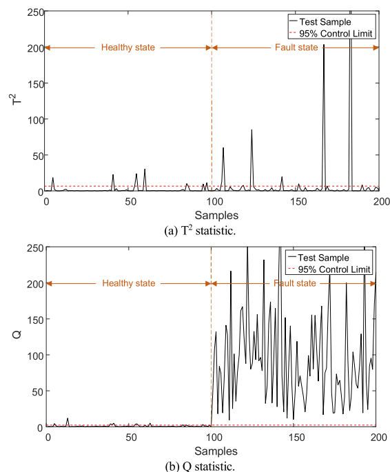
FIGURE 8. Experimental fault detection results of the proposed method under the same flow velocity condition.
