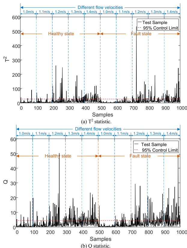
FIGURE 9. Experimental fault detection results of the method without denoising under different flow velocity conditions.
