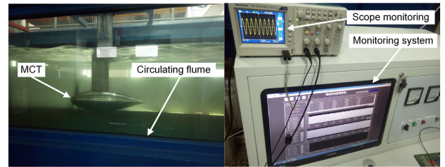
(a) The MCT in the circulating flume. (b) The monitoring system of the MCT.
