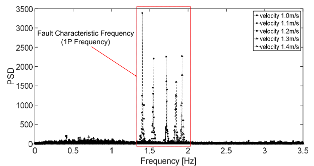
FIGURE 3. The MCT's fault characteristic frequencies in imbalance fault state under different flow velocity conditions.
