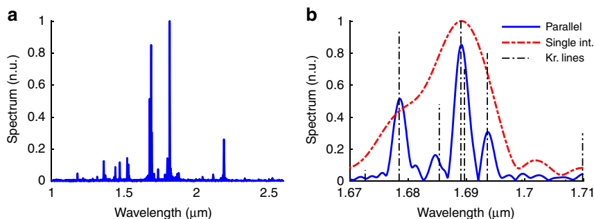
Fig. 5 Measured spectrum of the krypton source. a Krypton emission spectrum measured by the parallel interferometers. b Zoomed-in image of the wavelength range of 1.67–1.71 \mu\text{m} . The measured krypton peaks in the case of the four parallel interferometers (in blue) and single interferometer (in red) are shown. Reference lines of krypton are also plotted (dashed black lines)
