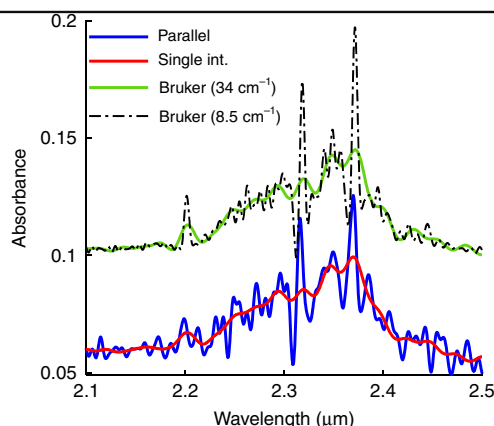
Fig. 6 Measured absorbance spectra of methane. Measured absorbance curves of methane measured by the parallel interferometers (in blue) and the single interferometer (in red) and compared to the absorbance measured by the benchtop spectrometer for the two corresponding resolutions
