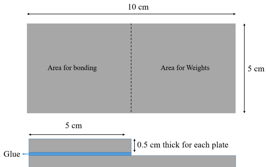
Figure 2: Top and side view of the specimen
