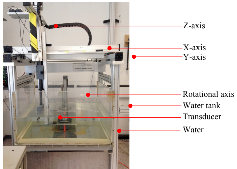
Figure 1: Ultrasonic device
