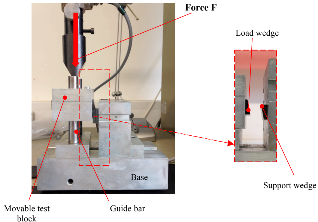
Figure 3: Shear device
