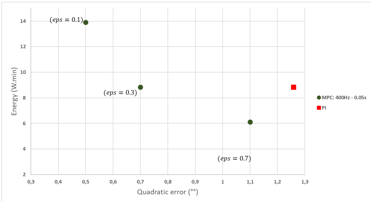
Figure 13: MPC/PI results
