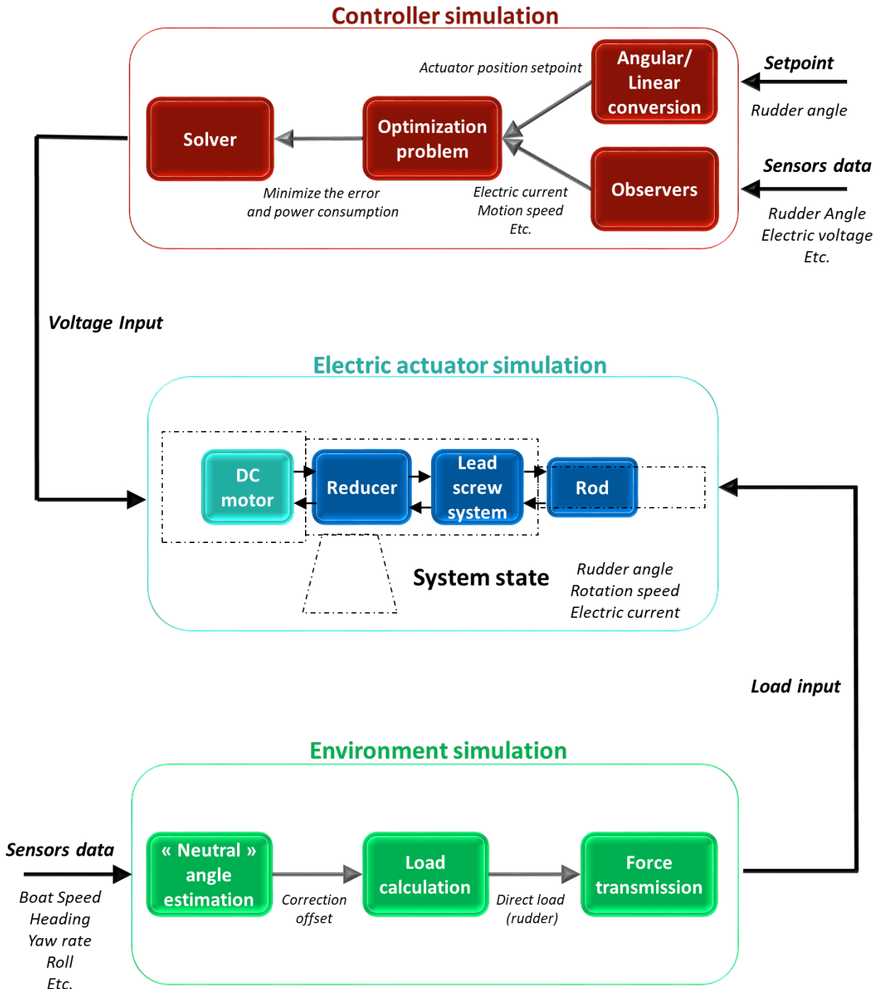
Figure 10: Simulation environment
