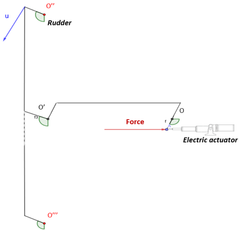
Figure 6: Rudder mechanism
