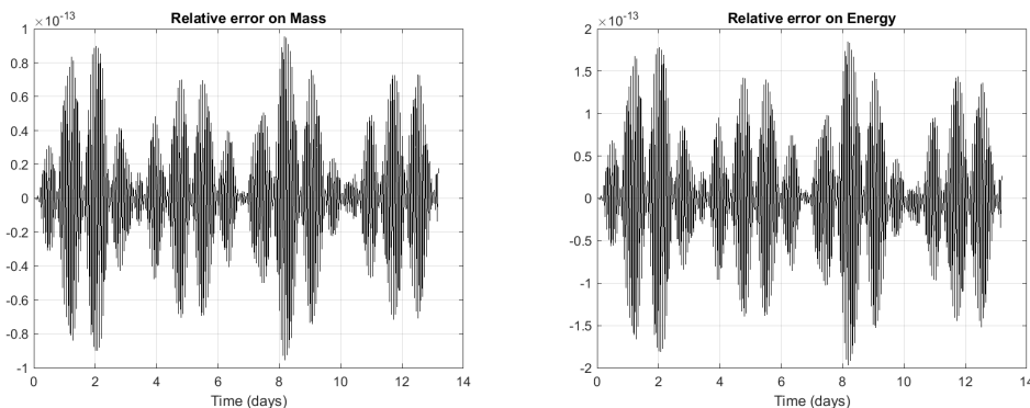
FIGURE 10. Test 1-a (barotropic EIG wave). Left panel: History of the mass relative error (33) for I_1 . Right panel: History of the energy relative error (33) for I_2 . The solver is the HCCS scheme in space with the ERK2 time scheme with CFL = 4 and 407 time iterations. The conservation accuracy is excellent in all cases, below 2.10^{-13} . The Cubed-Sphere grid is 6 \times 64 \times 64 .
