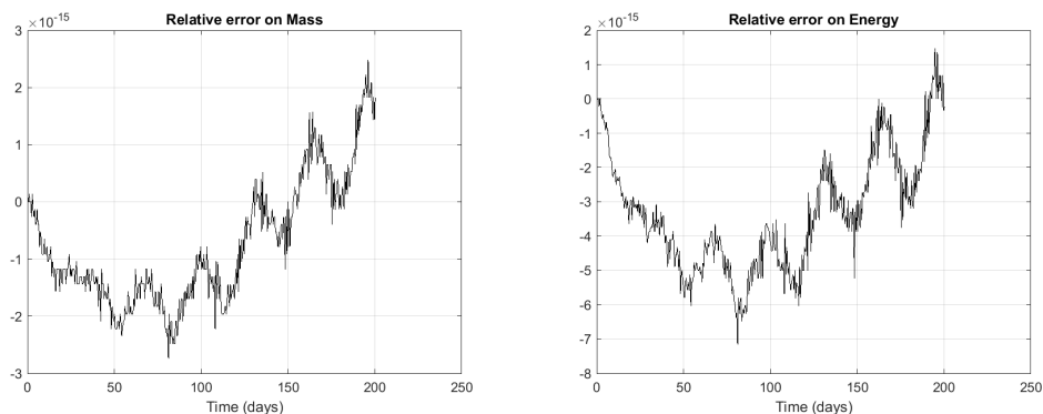
FIGURE 12. Test 2-a (baroclinic EIG wave). HCCS solver in space with the ERK2 time scheme with Courant number CFL = 5. Left panel: Mass relative error. Right panel: Energy relative error. In both case, the level is below 5 \cdot 10^{-15} , (machine accuracy). The Cubed-Sphere grid is 6 \times 64 \times 64 .
