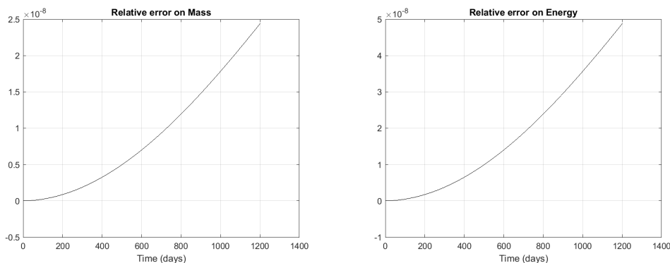
FIGURE 11. Test 1-b (barotropic Rossby wave). Mass and energy relative error (32). HCCS solver in space with ERK2 scheme time scheme with CFL = 16. The conservation accuracy is very good, even after 1203 days, (100 periods) with a level below 5 \cdot 10^{-8} in both cases. The Cubed-Sphere is 6 \times 64 \times 64 .
