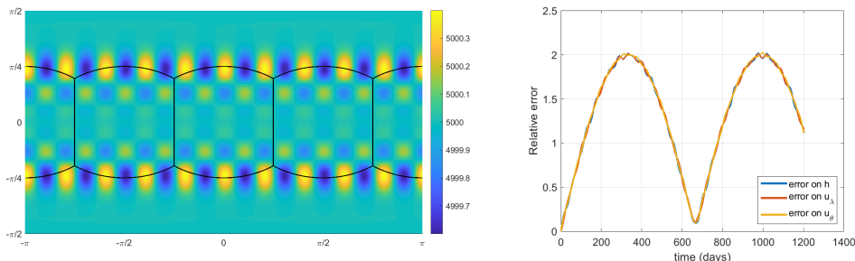
FIGURE 4. Test 1-b (barotropic Rossby wave), HCCS solver in space. The final time is t = 1203 days (100 periods). The time scheme is the ERK2 time scheme with 9289 time iterations and CFL = 16, see (21). Left panel: total h at final time. Right panel: history of the relative errors for h , u_\lambda (zonal velocity) and u_\theta (meridional velocity). The three curves are almost superposed. The resolution of the Cubed-Sphere is 6 \times 64 \times 64 .
