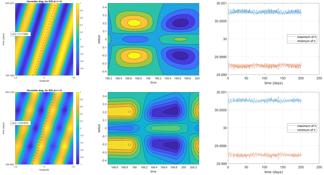
FIGURE 8. Test 2-a (baroclinic EIG wave). The HCCS solver in space is used. First line : RK4 time scheme with CFL = 1. Second line, ERK2 time scheme with CFL = 5. The first column represents time-longitude Hovmöller diagrams of the simulated solutions obtained by intersecting the zonal velocity at latitude \theta = 9 deg. The second column is a latitude-time Hovmöller diagram obtained by intersecting the zonal velocity at \lambda = -18 deg. The third column displays the maximum and minimum values of the total height h over the full simulation (final time: 190 days). The distortion in the middle panel, bottom line, is attributed to the Courant number CFL = 5. The Cubed-Sphere is 6 \times 64 \times 64 .
