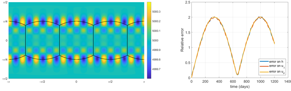
FIGURE 4. Test 1-b (barotropic Rossby wave), HCCS solver in space. The final time is t = 1203 days (100 periods). The time scheme is the ERK2 time scheme with 9289 time iterations and \text{CFL} = 16 , see (20). Left panel: total h at final time. Right panel: history of the relative errors for h , u_\lambda (zonal velocity) and u_\theta (meridional velocity). The three curves are almost superposed. The resolution of the Cubed-Sphere is 6 \times 64 \times 64 .
