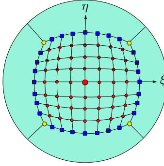
FIGURE 1. The points of a typical panel of the Cubed-Sphere are classified in three categories as follows: (i) the (N-1)^2 circles correspond to the internal points; (ii) the 4(N-1) squares correspond to the edge points ; (iii) the 4 pentagons correspond to the corner points. The coordinate system consists of the two "equatorial" angles (\xi, \eta) , -\pi/4 \leq \xi, \eta \leq \pi/4 , with origin at the panel center. The angles \xi is analog to the longitude angle \lambda . The angle \eta is also a "longitude" angle, deduced from \xi by a 90 degrees rotation.
