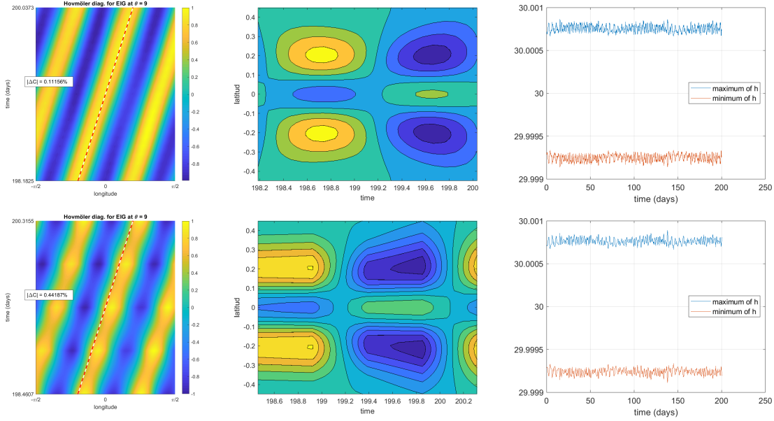
FIGURE 8. Test 2-a (baroclinic EIG wave). The HCCS solver in space is used. First line : RK4 time scheme with \text{CFL} = 1 . Second line, ERK2 time scheme with \text{CFL} = 5 . The first column represents time-longitude Hovmöller diagrams of the simulated solutions obtained by intersecting the zonal velocity at latitude \theta = 9 deg. The second column is a latitude-time Hovmöller diagram obtained by intersecting the zonal velocity at \lambda = -18 deg. The third column displays the maximum and minimum values of the total height h over the full simulation (final time: 190 days). The distortion in the middle panel, bottom line, is attributed to the Courant number \text{CFL} = 5 . The Cubed-Sphere is 6 \times 64 \times 64 .
