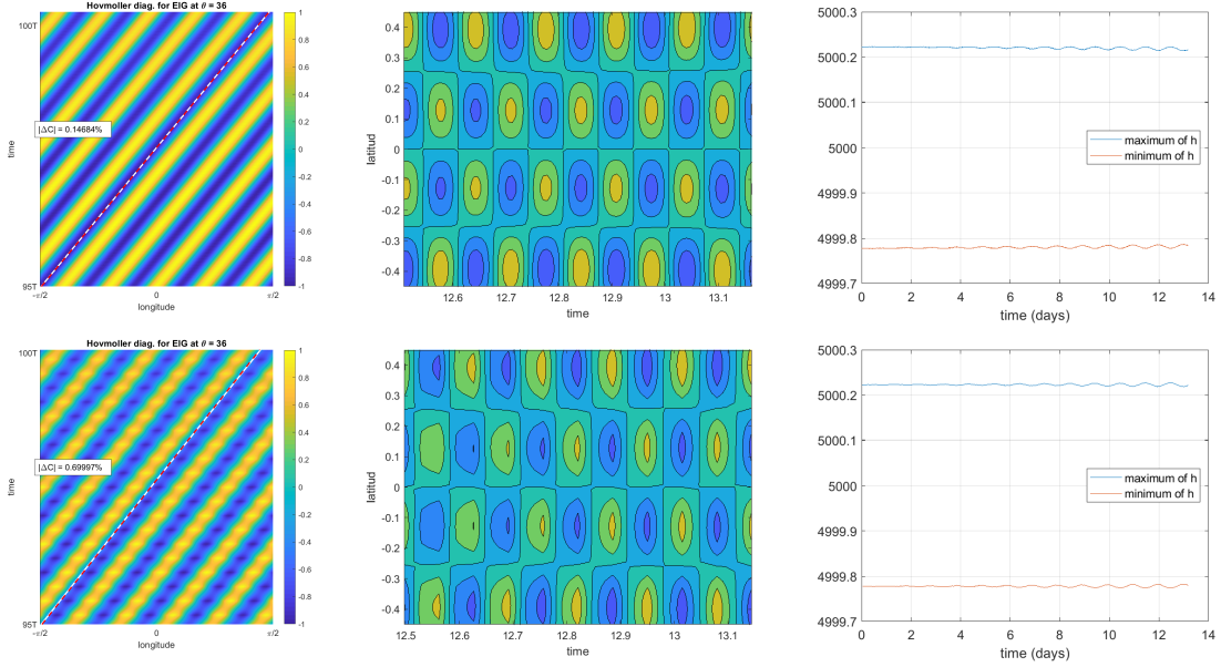
FIGURE 3. Test 1-a (barotropic EIG wave). HCCS solver in space at final time is t = 13.5 days. First line : RK4 time scheme at \text{CFL} = 0.9 . Second line, ERK2 scheme at \text{CFL} = 4 . The first column corresponds to time-longitude Hovmöller diagrams of the numerical solutions obtained by intersecting the zonal velocity at latitude \theta = 36 deg. The second column is corresponds to latitude-time Hovmöller diagrams obtained by intersecting the zonal velocity at longitude \lambda = -18 deg. The third column displays the maximum and the minimum history of the total height h over the full simulation. No significant damping is observed. The Cubed-Sphere resolution is 6 \times 64 \times 64 .
