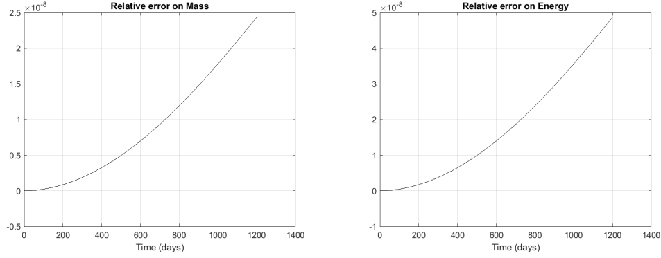
FIGURE 11. Test 1-b (barotropic Rossby wave). Mass and energy relative error (31). HCCS solver in space with ERK2 scheme time scheme with CFL = 16 . The conservation accuracy is very good, even after 1203 days, (100 periods) with a level below 5.10^{-8} in both cases. The Cubed-Sphere is 6 \times 64 \times 64 .
