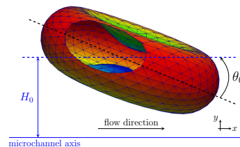
Fig. 17. Schematic representation of the initial configuration of a biconcave red blood cell (colors on the membrane represent |\kappa| ), where H_0 and \theta_0 are respectively the initial offset position of its centroid relative to the flow axis and the initial inclination angle measured from its flat plane to the axis of the flow.
