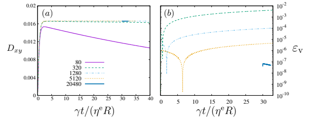
Fig. 9. Temporal evolution of (a) the Taylor deformation parameter D_{xy} and (b) the relative derivation of the enclosed volume \epsilon_v = V/V_0 - 1 of a drop in a capillary flow ( Ca = 0.05 and \beta = 0.8 ) as a function of the number of elements N used on the drop surface.
