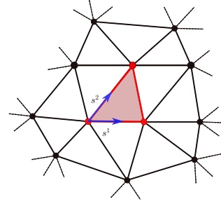
Fig. 4. A Loop element (shaded triangle) with its local parametrization \mathbf{s} = (s^1, s^2) and its one-ring elements (bounded by solid lines), forming a regular Loop's patch containing 12 control vertices.
