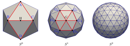
Fig. 2. An illustration of Loop's subdivision rule from the initial control mesh S^0 (an icosahedron) to S^1 mesh (after one refinement) and S^2 mesh (after two refinements).
