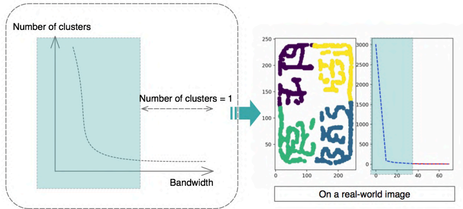
Figure 8. Visualization of clustering results under different bandwidths.
