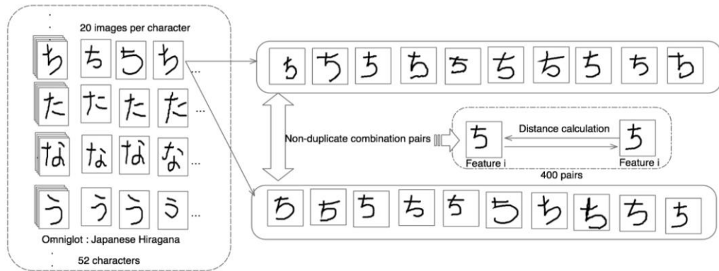
Figure 17. Experiment on feature and distance calculation method selection.
