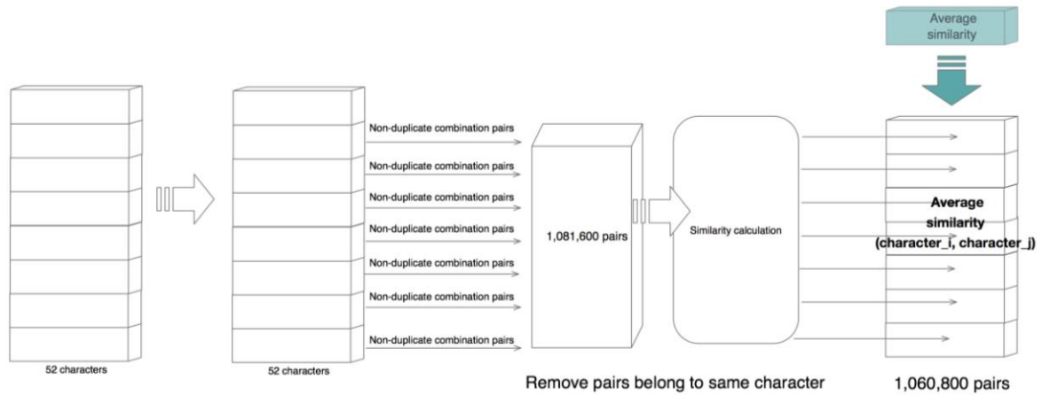
Figure 20. Calculating the distinction score of each character.
