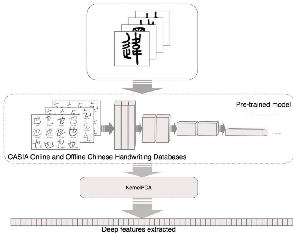
Figure 11. Extraction of CNN features.
