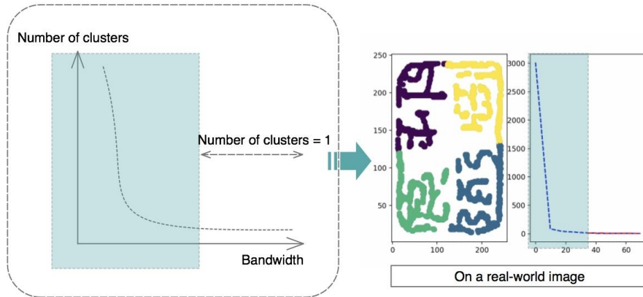
Figure 8. Visualization of clustering results under different bandwidths.
