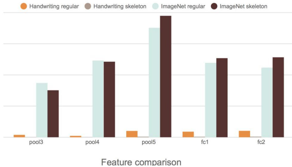
Figure 22. Score_{feature_i} in different situations.
