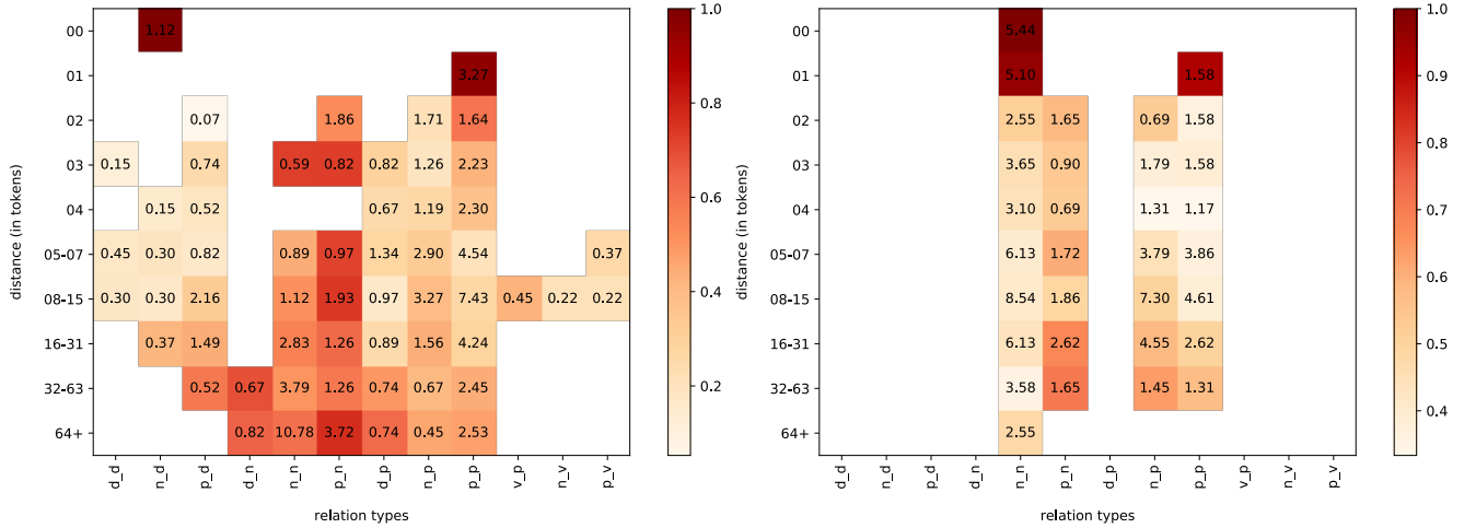
(a) Spurious relation in Democrat (89.7% of the errors are explained). (b) Spurious relation in ANCOR (92.3% of the errors are explained).
