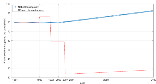
Figure 4. The fluvial sediment supply to the coast over the period 1954–2100 under the combined effect of climate change and human impacts (red line) and under natural forcing only, including climate change (blue circles).
