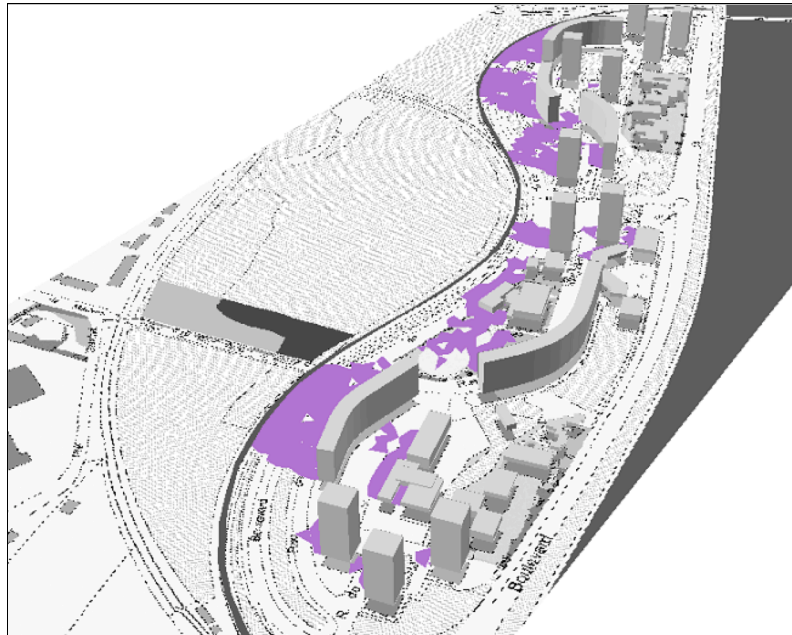
Figure 4 : Example of synthetized map: areas of discomfort in external space (crossing of wind and solar indicators)
