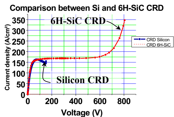
Fig 2. CRD simulated characteristics.
