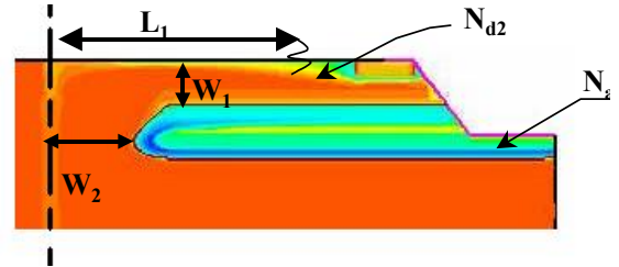
Fig. 4. VJFET parameters to be optimized.
