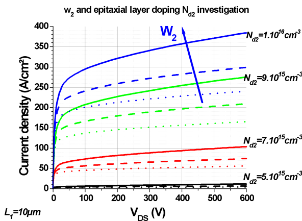
Fig.5-a Epitaxial layer investigation
