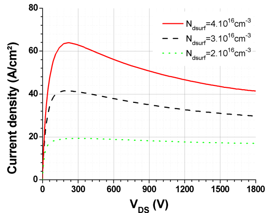
Fig.5-b Surface channel adjustment.
