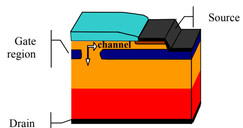
Fig.3 Cross section of the VJFET
