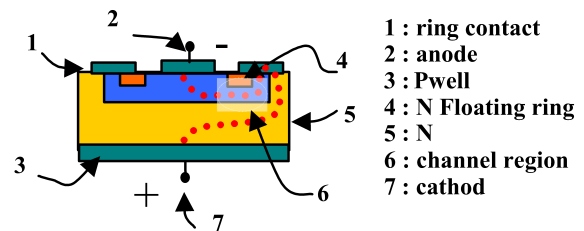
Fig. 1 Cross section of a silicon CRD.
