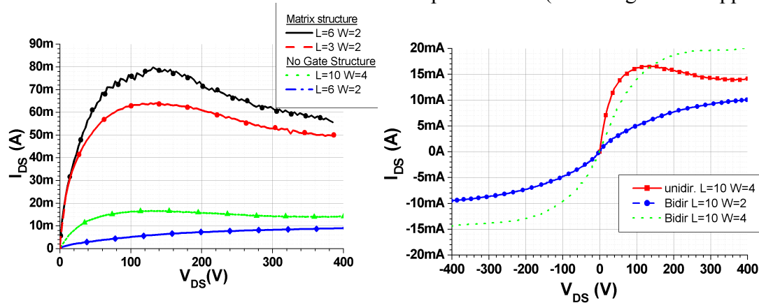
Fig.7. Electrical measured characteristics.
