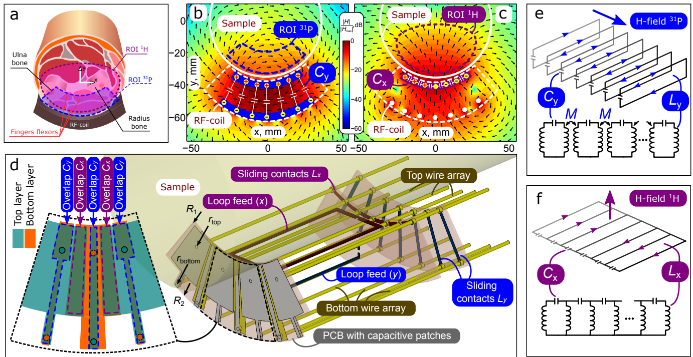
Fig. 1. Application and practical realization of proposed dual-nuclei coil: (a) target regions of interest at ^{31}\text{P} (81 MHz) and ^1\text{H} (200.1 MHz) covering flexor muscles of a human arm; capacitive interconnection of wire ends and corresponding orthogonal-polarized eigenmodes of dual-stage wire array: (b) volume mode for ^{31}\text{P} , (c) surface mode at ^1\text{H} ; (d) practical realization of the proposed coil (inset on the left demonstrates the layout of PCB with capacitive patches for interconnection of wires); (e) wire currents of volume mode and its equivalent circuit; (f) wire currents of surface mode and its equivalent circuit.
