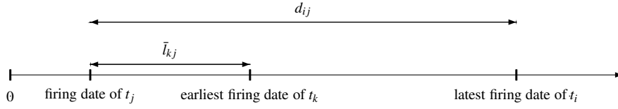
Fig. 4 Condition C2 of SC: \bar{l}_{kj} \leq d_{ij} for t_i \in G(\alpha), t_j \in En(M), t_k \in CFS(t_i)
