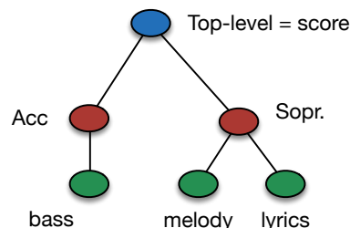
Figure 7. Structure of the example score
