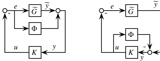
Figure 8. Stability of the closed-loop (\widetilde{G} + \Phi, K) is equivalent to stability of the closed-loop (\widetilde{G}, \text{feedback}(K, \Phi)) . See also [23].
