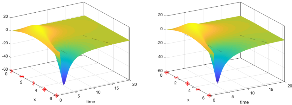
Figure 5. Model matching. Simulation of optimized reduced-order system (left) with K_0 based on (9) and infinite-dimensional system (right) with H_\infty -optimal controller K^* based on (12). The intermediate result on the left leads to the final result on the right. The stars '*' indicate sensor positions.
