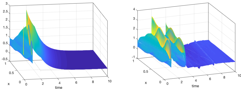
Figure 9. Wave equation. Simulations with nonzero initial condition for K obtained by backstepping control (left) and K^* = K_0 + K obtained by optimizing \text{feedback}(\widetilde{G}, \widetilde{K}) via systeme (right). Both controllers are infinite-dimensional, but implementable.
