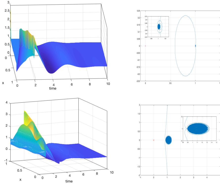
Figure 10. Wave equation. Finite-dimensional controllers obtained by mixed sensitivity in (20). Top left initial K_0 . Bottom left optimal K^\# = K_0 + K_1(\mathbf{x}^\#) . Top right, Nyquist plot 1 + (K(\mathbf{x}_0) - K_0)G_0 does not encircle origin, bottom right Nyquist plot 1 + (K(\mathbf{x}^\#) - K_0)G_0 .
