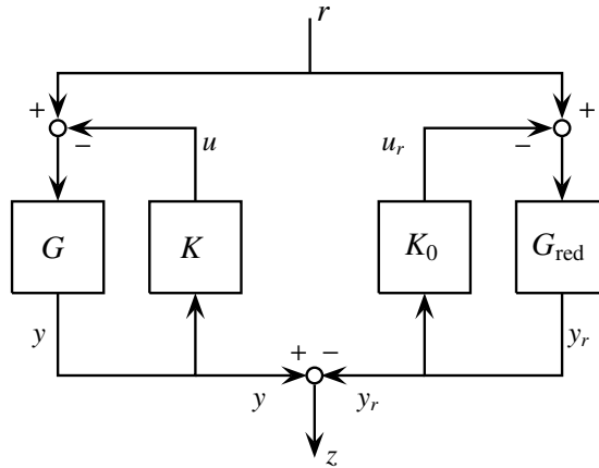
Figure 3. Model matching step (b). H_\infty -optimization of channel r \rightarrow y - y_r in (11) starting at initial guess K = K_0 leads to overall optimal K = K^* and is a special case of (3). In the reference model on the right K_0 obtained in step (a) remains now fixed.
