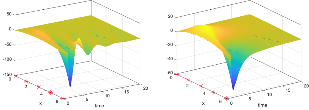
Figure 6. Mixed sensitivity. Simulation with K^* \in \mathcal{K}_2 obtained with weight W_e^{(1)} (left). States near \xi = L show undesirable transient oscillations. Simulation with K^{**} obtained with W_e^{(2)} (right) proves satisfactory.
