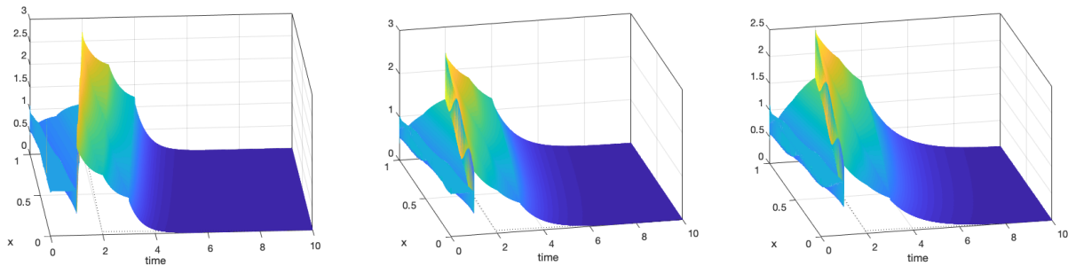
Figure 14. Method 2. \bar{K}(q) = \bar{K}_{\text{nom}} + (q-3)\bar{K}_1 + (q-3)^2\bar{K}_2 and K(q) = K_0 + \text{feedback}(\bar{K}(q), \Phi(q)) . Simulations for q = 2, 3, 4
