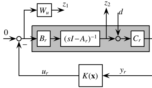
Figure 2. Model matching. Preliminary stabilization via structured H_2 -synthesis using P_{\text{red}} with channel d \rightarrow z_r = (z_1, z_2) = (W_u u_r, x_r) .
