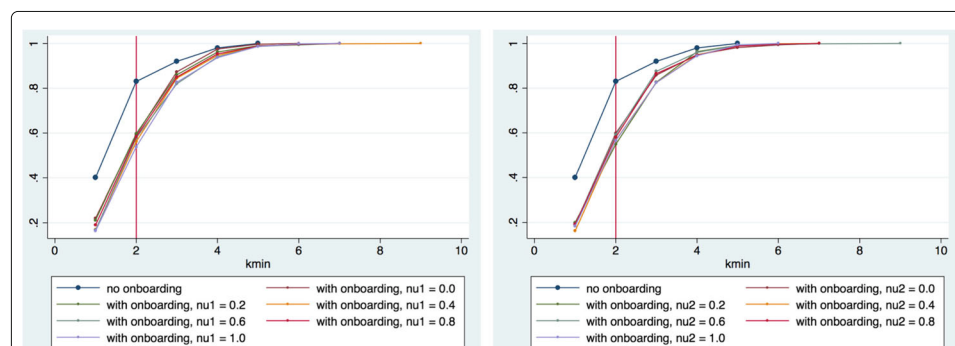
Fig. 4 Cumulate Density Functions of the average value of k_{\min} that minimizes the Kolmogorov-Smirnov distance between the in-degree distribution of each interaction network and its best-fit power-law model in the control and treatment groups. Twenty percent of the networks evolved without onboarding (dark blue) have degree distributions that test negatively for H1. When onboarding is introduced, that percentage rises to between 50 and 90%. On the left , the treatment group interaction networks have been grouped according to the value taken by \nu_1 ; on the right , they have been grouped according to the value taken by \nu_2
