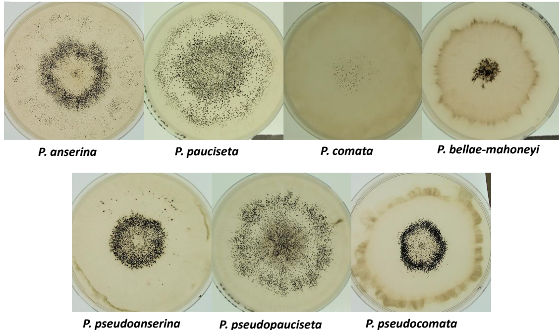
Figure 19 Perithecium production patterns of the species from the P. anserina species complex are species-specific . The medium is the minimal M2 medium with 4g/L of potato dextrins. On other media, the strains will exhibit different patterns.
