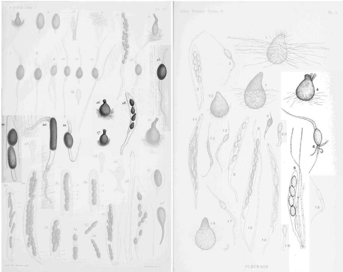
Figure 17 Two early drawings of P. anserina . Left (fig. 15-21), by E.C. Hansen in 1876 under the name Sordaria anserina ; Right (fig. 4-6) by D. Griffiths in 1901 under the name Pleurage anserina . Compare the right drawings with those of Traverso (figure 14).
