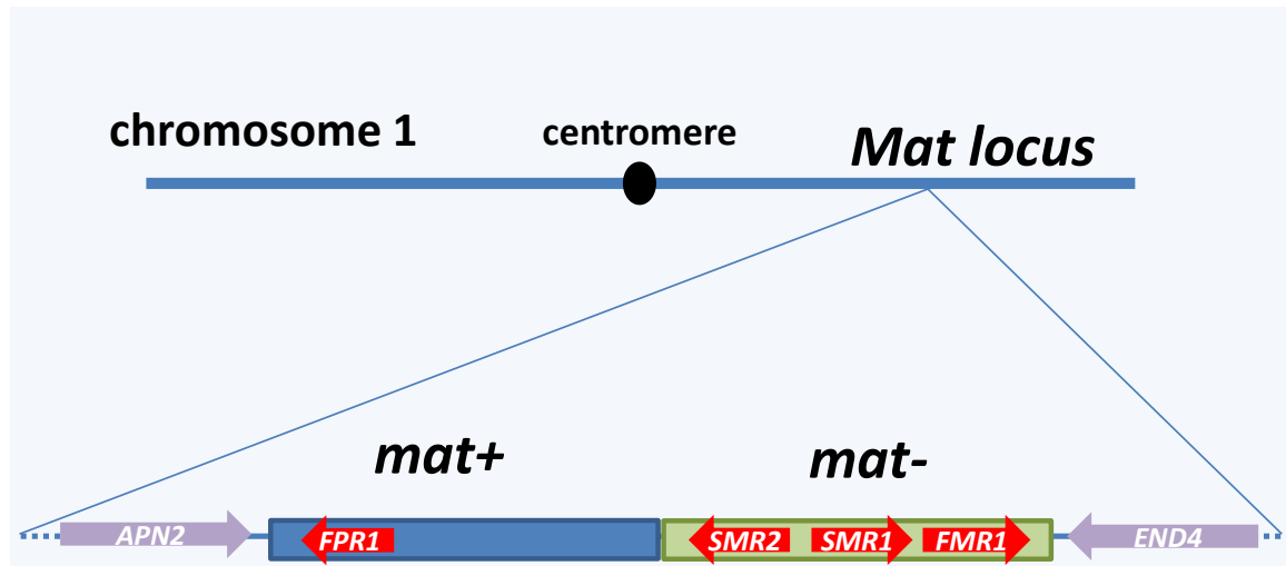
Figure 88 Structure of the mating type locus of the mat+ / mat- dual mater strain PM154
