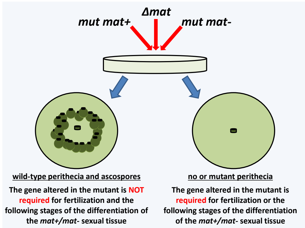
Figure 59 Trikyon analyses with \Delta mat to study development in P. anserina . see text for detail.
