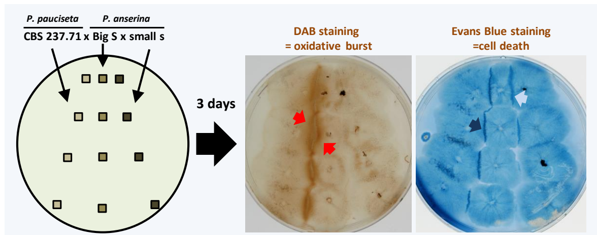
Figure 80 Lack of Hyphal Interference between strains of P. anserina and presence of hyphal interference between P. anserina and P. paucisetata . Podospora paucisetata CBS 237.71 and the BIG S and small s strains of P. anserina were inoculated along diverging lines as indicated on the left scheme. After three days, the DAB staining shows a lack of oxidative burst when the BIG S and small s strains of P. anserina are confronted; yet cell death due to vegetative incompatibility (light blue arrow) occurs at the confrontation between the two vegetatively-incompatible strains of P. anserina as shown by the Evans Blue staining. On the contrary, an intense oxidative burst on both P. anserina and P. paucisetata mycelia (red arrows) occurs at the junction between P. anserina and P. paucisetata , along with many hyphal death (dark blue arrow).
