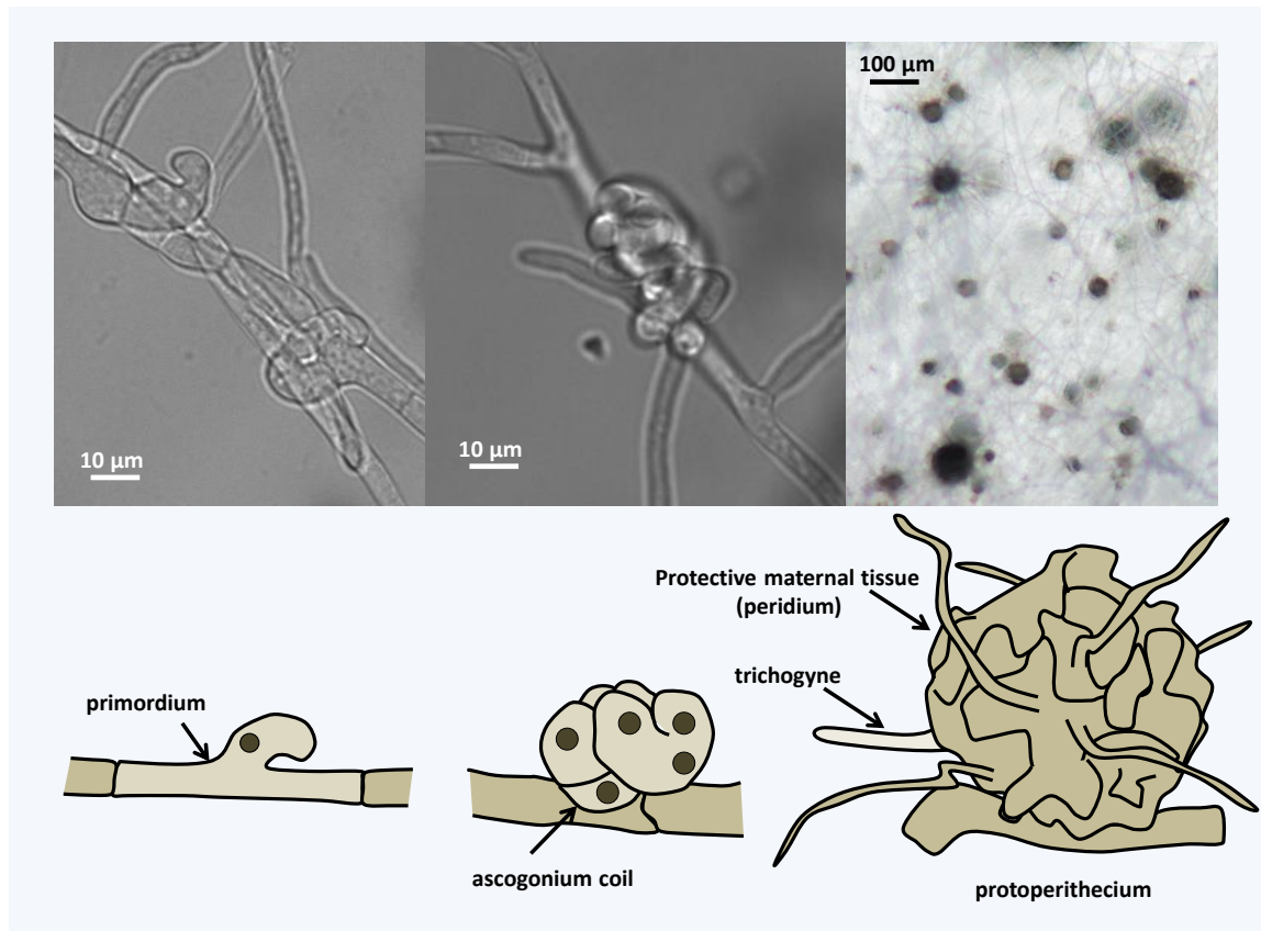
Figure 39 Differentiation of the P. anserina female gametangium. The fertile tissue is colored in a lighter color compared to the maternal one. See text for description.
