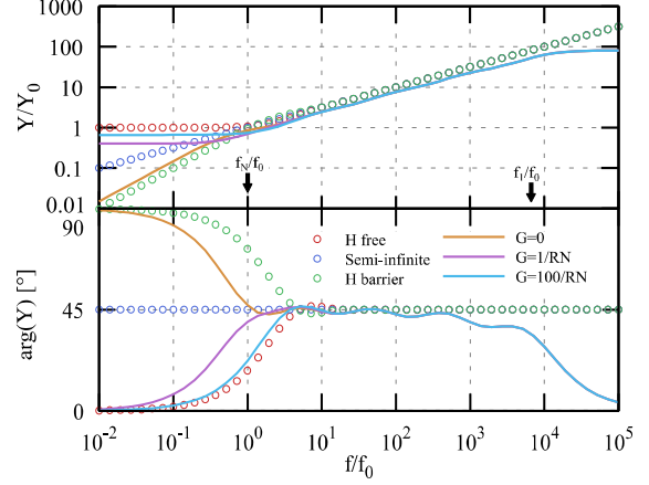
Fig. 5: Bode-like representation of normalized "Admittance" \tilde{Y}(f)/Y_0 of diffusion through oxide for the theoretical model (symbols, three cases according to second interface properties) and for the RC-ladder (lines) model for \alpha_R = 3 and N = 5 ; Arrows indicating the domain of validity.
