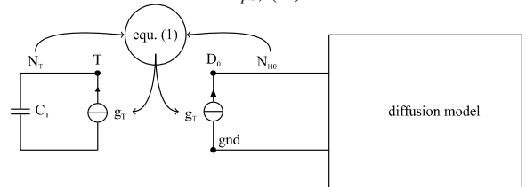
Fig. 3: Organization of the R-D and Diffusion model implementation.
