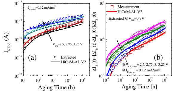
Fig. 10: Comparison between measurement and HiCuM-AL-V2 simulation: (a) I_{REPS} and (b) excess base current ( \Delta I_B / I_{B0} ) under J_{E, stress} of 0.12, \text{mA}/\mu\text{m}^2 for different V_{CB, stress} .
