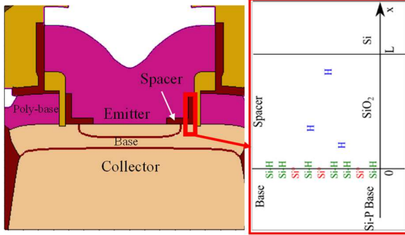
Fig. 2: Schematic of the hydrogen diffusion model considering the interface between the base and the EB-spacer; L is the E-B spacer thickness.
