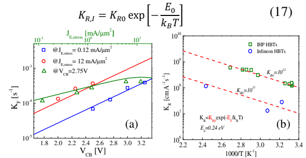
Fig. 12: Evolution of (a) K_{F,I} for different V_{CB, stress} and J_{E, stress} and (b) K_{R,I} as a function of the inverse of junction temperature.
