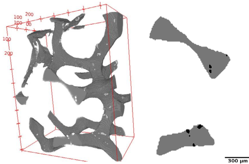
Fig. 5. Local tomography visualization of inter-metallic particles inside an ERG foam. (a) Shows a 3D rendering and (b) a reconstructed tomographic slice. In (a) the particles are visible in white. They are black in (b).
