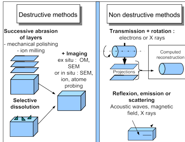
Fig. 2. General panorama of the methods available to obtain 3D images of a microstructure (scanning acoustic microscopy, SAM) or magnetic (Nuclear Magnetic Resonance, NMR) waves can alternatively be used for such probing.
