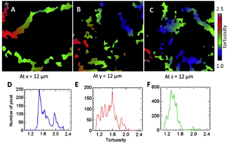
Fig. 6. (Color online.) From [34]. “Tortuosity distribution” of a \text{LiCoO}_2 sample shown as (A–C) spatial distribution maps and also (D–F) histograms for all three directions along the positive direction
