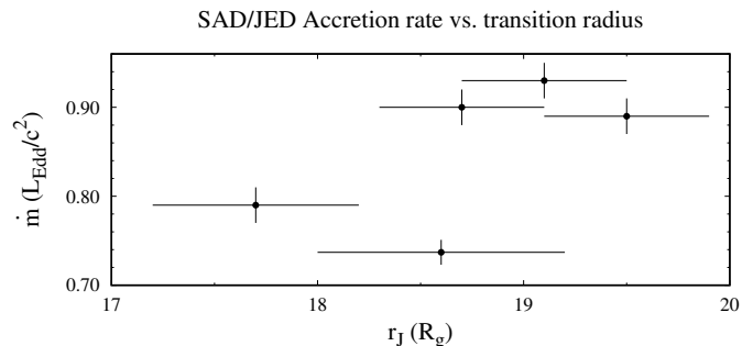
Fig. 16. Accretion rate vs. transition radius of the SAD–JED model for the different observations (see Table 5).
