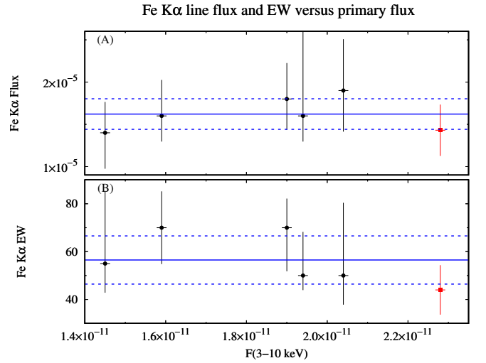
Fig. 8. Parameters of the Fe K\alpha line plotted against the primary flux in the 3\text{--}10 keV band. The red square corresponds to the 2004 XMM-Newton observation. Panel A : line flux in units of photons \text{cm}^{-2} \text{s}^{-1} . Panel B : line equivalent width in units of eV. Error bars denote the 1\sigma uncertainty. The blue solid lines represent the mean value for each parameter during the campaign, while the blue dashed lines represent the standard deviation.
