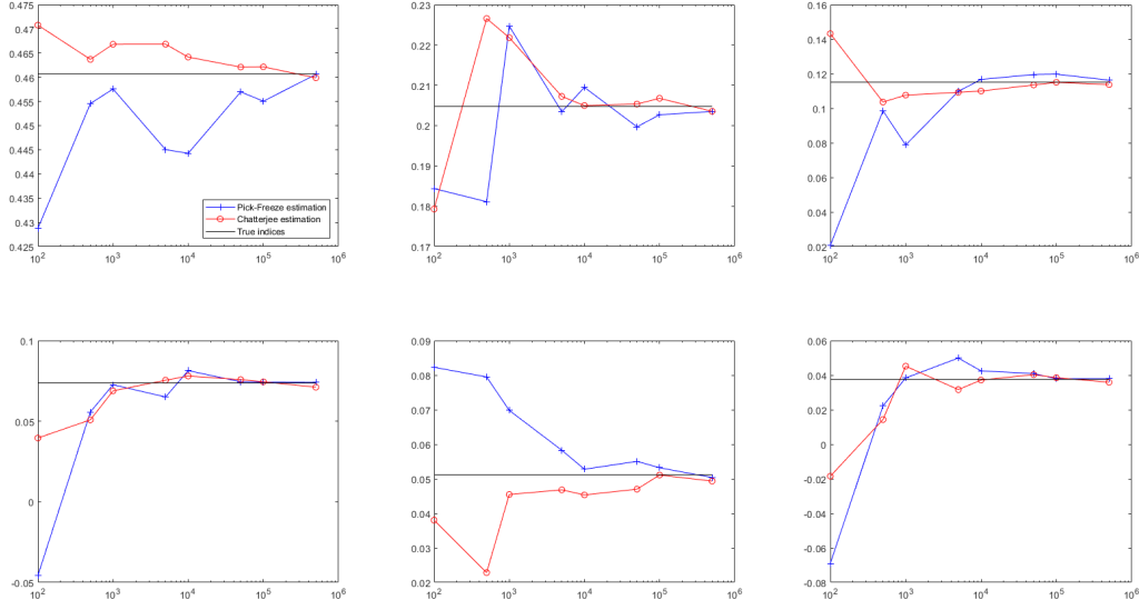
Figure 1: The Sobol g -function model (27). Convergence of both methods when N increases. The sixth first-order Sobol indices have been represented from left to right and up to bottom. Several sample sizes have been considered: N = 100, 500, 1000, 5000, 10000, 50000, 100000 , and 500000 for the Pick-Freeze estimation procedure and correspondingly (p + 1)N for the estimation procedure proposed in [9]. The x -axis is in logarithmic scale.
