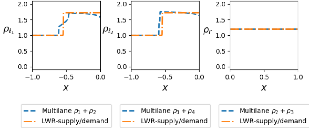
Figure 8: In each picture, the dashed blue line is the sum of the solutions to the multilane model (3.1)–(3.5)–(3.8): from left to right, lanes 1 and 2; lanes 3 and 4; lanes 2 and 3. The dash-dotted orange line corresponds to the solution to the LWR model (2.1), obtained through a Godunov type scheme, with priorities (1/2, 1/2) : from left to right, incoming roads a , b , outgoing road c . The initial data are given in (4.5) and (4.6) respectively. In each lane we set V = 1.5 .
