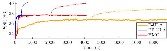
Fig. 3. PSNR along time for Simu1. Dotted lines indicate the PSNR of the MMSE estimator of the TRF after the burn-in regime.
