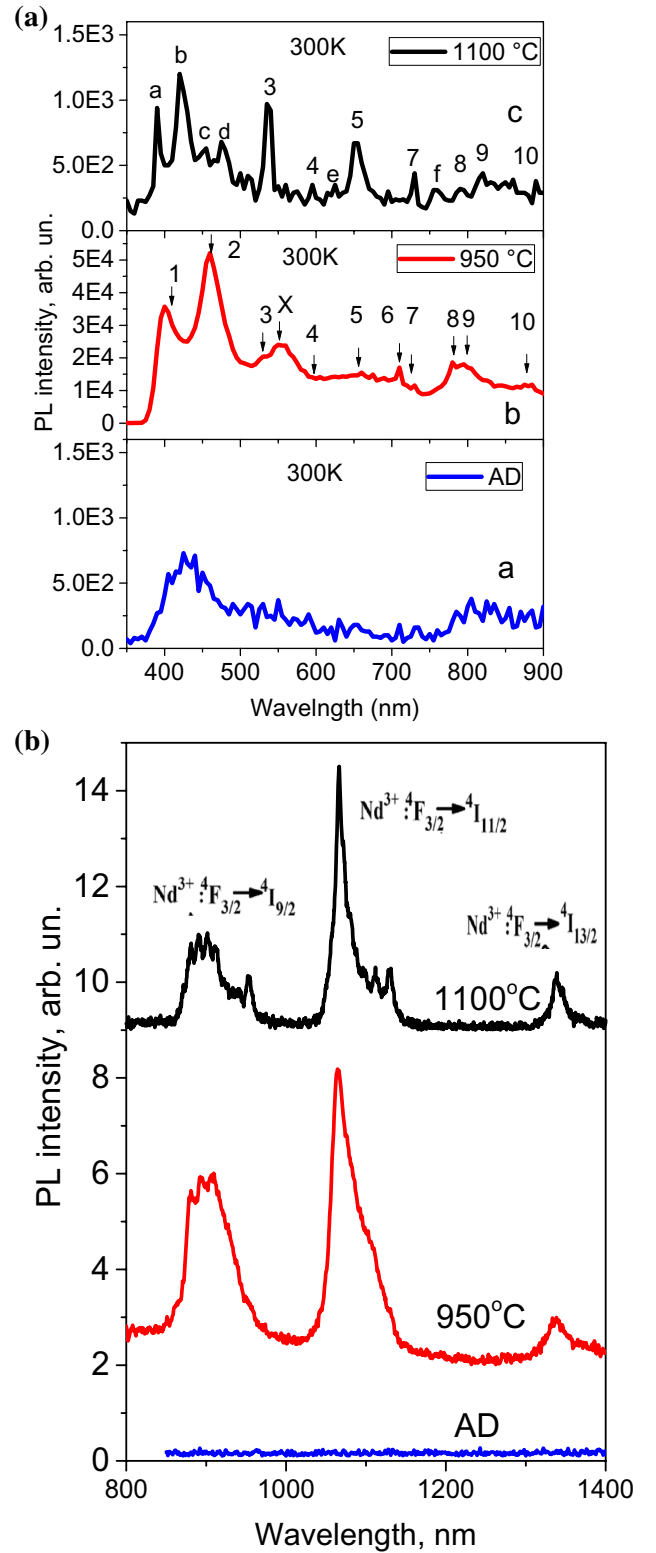
Fig. 4 PL spectra of Si-HfO 2 :Nd films: as-deposited and annealed at 950 and 1100 °C recorded in the visible (a) and infrared (b) spectral ranges
