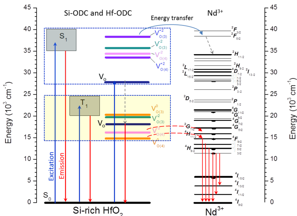
Fig. 7 Schematic presentation of different radiative centers and possible ways for energy transfer towards \text{Nd}^{3+} ions. Si-ODC and Hf-ODC are oxygen vacancies (oxygen deficient centers) located in \text{SiO}_2 (and/or \text{SiO}_x ) and \text{HfO}_2 phases
