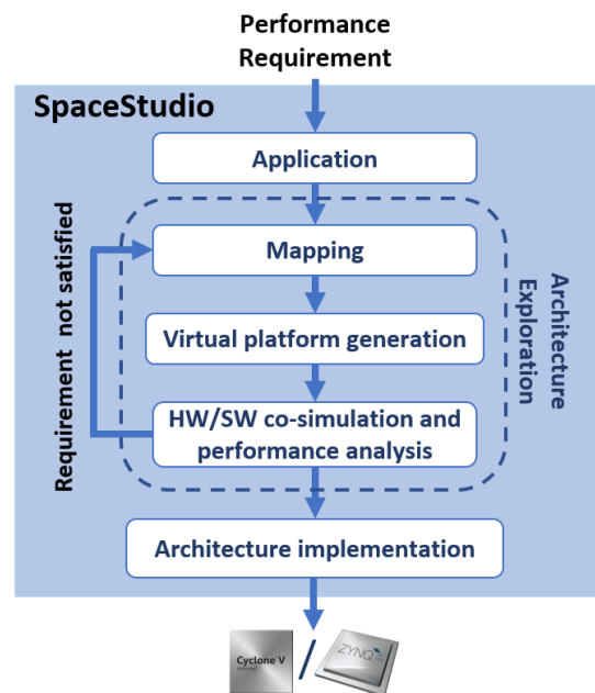
Fig. 2. SpaceStudio workflow
