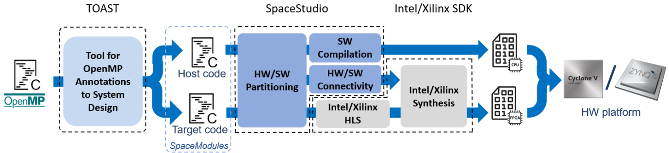
Fig. 1. From OpenMP to SoC FPGA workflow (TOAST stands for Tool for OpenMP Annotations to System design Translation )
