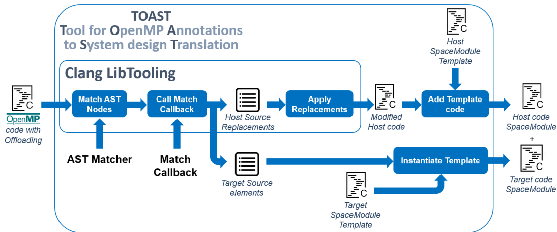
Fig. 3. TOAST Architecture
