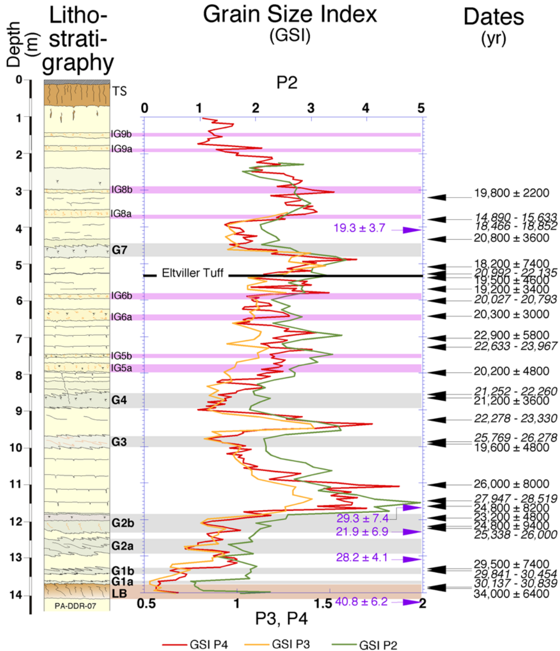
Figure 2. Nussloch P4 loess sequence. (left) Lithostratigraphy of the dilated part of the record (yellow, loess; brown-red, cambisol; light grey blue, tundra gley) [Antoine et al. , 2001, 2002]. (middle) Grain-size index (GSI) records from the P2, P3 and P4 profiles, showing a great similarity. GSI was calculated for P2 as (20-50 \mu\text{m}) / <20 \mu\text{m} , based on sieve and pipette grain-size analyses, and for P3 and P4 as (52.6-26 \mu\text{m}) / <26 \mu\text{m} , based on laser Coulter analyses. P2 and P3 depths were tuned to P4 by correlating the observed lithological units, except for the Eltviller tuff (ET, volcanic ash), which was used as an independent marker to test the tuning. Horizontal bands mark the cambisol (brown), the main gleys (green) and the less developed gleys or oxidized horizons (violet). (right) All available dates: ^{14}\text{C} (italic) and luminescence dates obtained on the P4 (in purple) and P2 (the rest). AMS dates, determined on preserved organic matter and indicating the plant degradation, have been converted to calendar years by using Calib05 [Bard et al. , 1998; Reimer et al. , 2004]. Only the luminescence dates, corresponding to the burial of dust grains in the sediment, are used to validate our age model.
