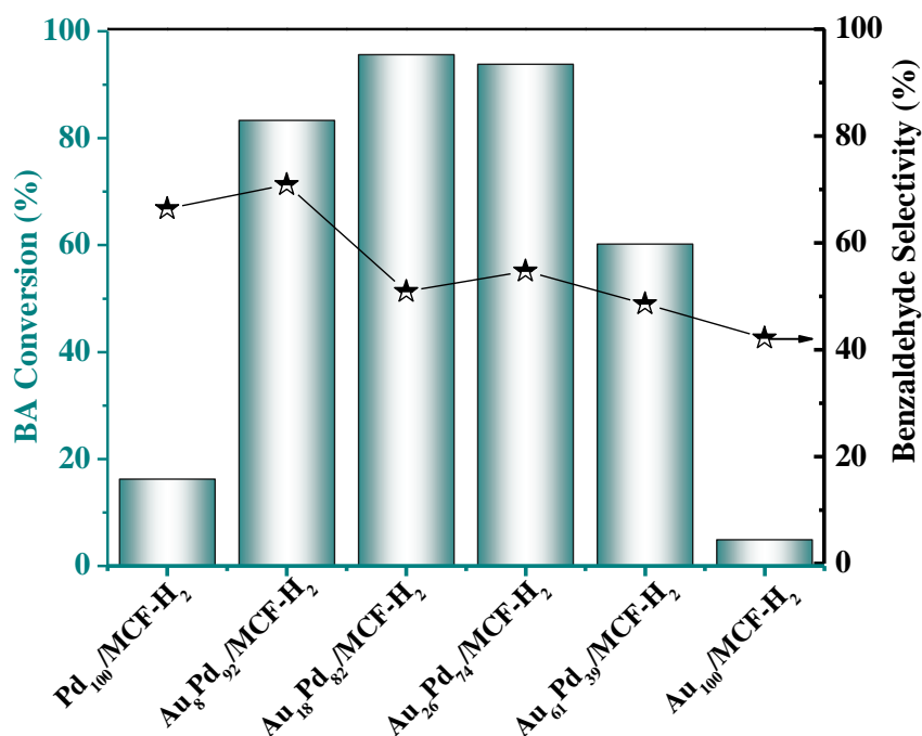
Fig. 9. Selectivity and conversion on catalysts in the benzyl alcohol partial oxidation reaction.
