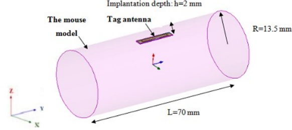
Figure 2. Implanted tag in the homogeneous body phantom.
