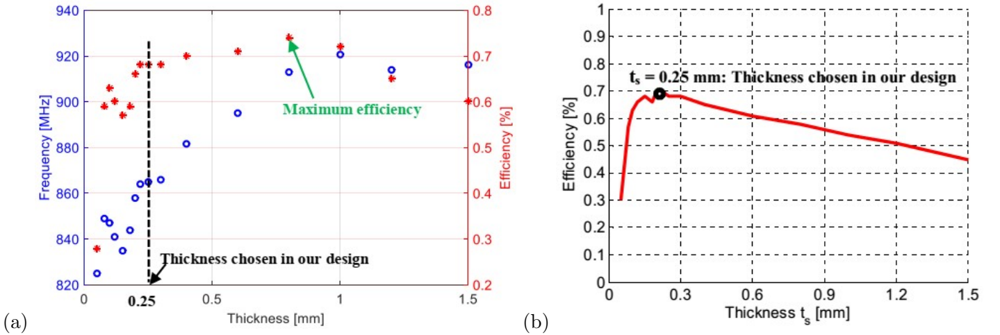
Figure 7. Simulation as a function of the insulation layer thickness t_s : (a) Efficiency and resonance frequency of the antenna, (b) Antenna efficiency at 868 MHz.
