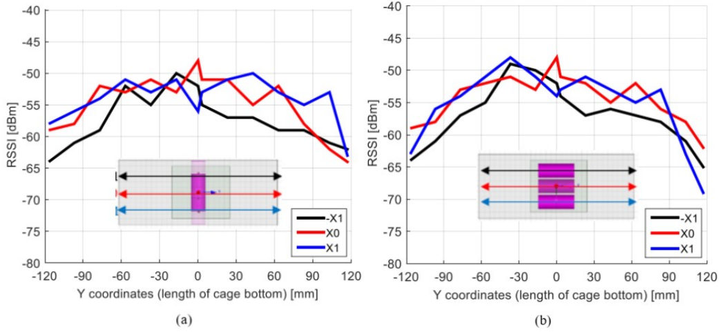
Figure 19. RSSI measurements when the phantom model is oriented along the X axis (a), and along the Y axis (b) versus the position of the phantom along the Y axis.
