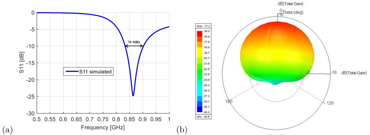
Figure 9. Simulated results of the implanted antenna with insulation layer: (a) Reflection coefficients, (b) Radiation pattern.
