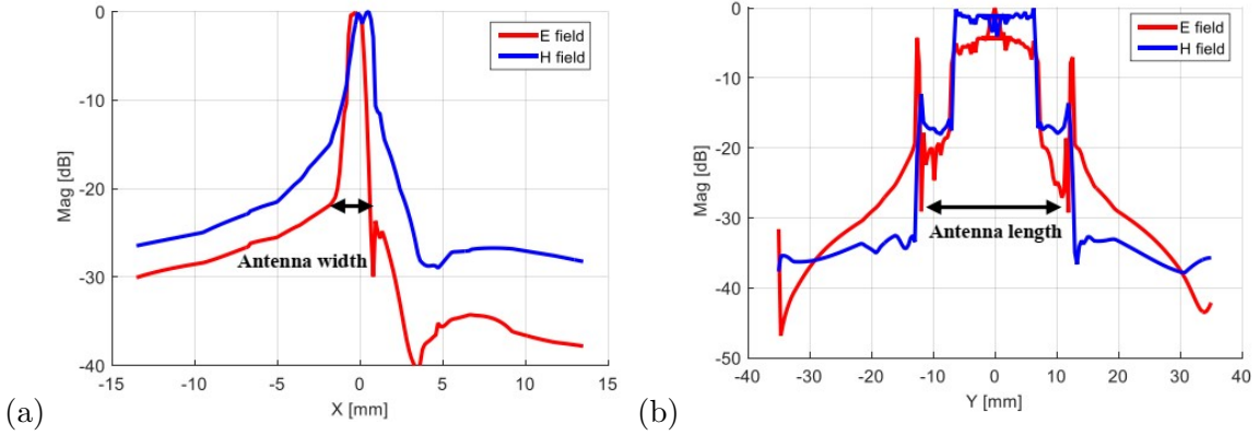
Figure 20. E and H standardized fields as a function of the width of the homogeneous model : (a) Along the X axis, (b) Along the Y axis.
