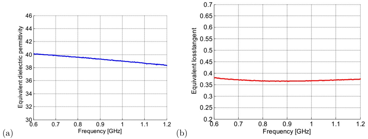
Figure 13. Measurement results of the equivalent homogeneous mouse tissue: (a) The equivalent dielectric permittivity, (b) The equivalent loss tangent.
