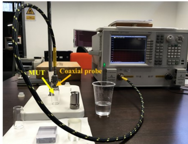
Figure 12. Equivalent dielectric permittivity measurement set-up.
