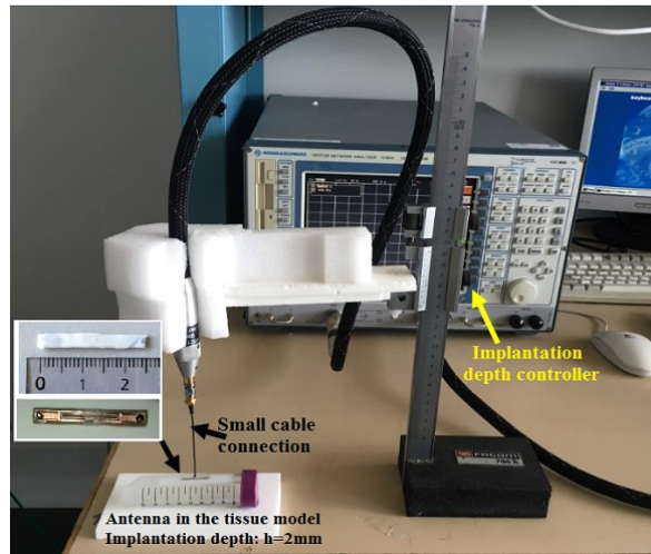
Figure 10. Reflection coefficient measurement set-up.
