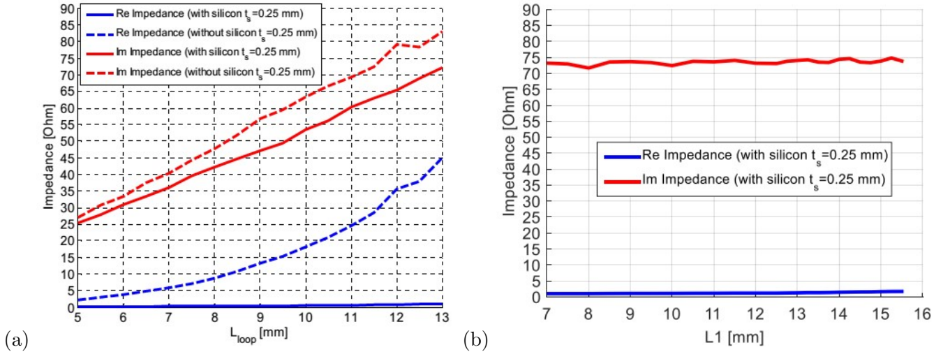
Figure 5. Simulated at 868 MHz: (a) Loop impedance as function of its length L_{loop} for W_{loop}=1 mm, (b) Antenna impedance as function of the dipole length L1 for L_{loop}=13 mm.
