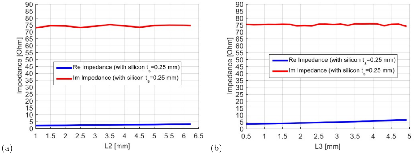
Figure 6. Antenna impedance at 868 MHz: (a) As function of the parameter L2 for L1=12.5 mm, (b) As function of the length L3 of the metal plates for L1 = 12.5 mm and L2 = 8.1 mm.
