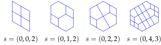
Figure 6: Some geometric realizations of s -permutahedra in dimension 2.
