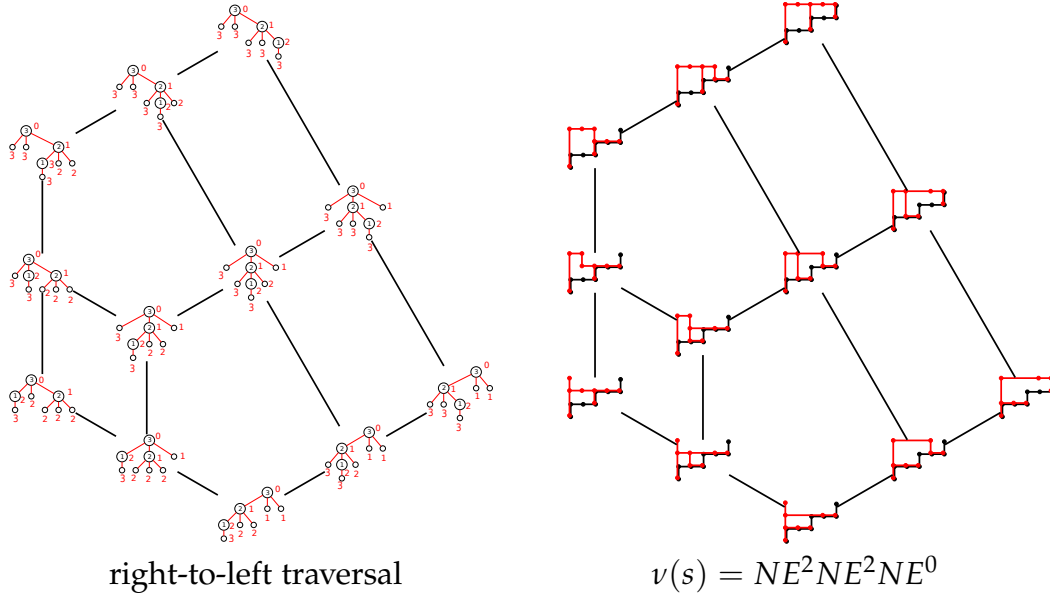
Figure 5: The s -Tamari lattice and the \nu(s) -Tamari lattice for s = (0, 2, 2) .
