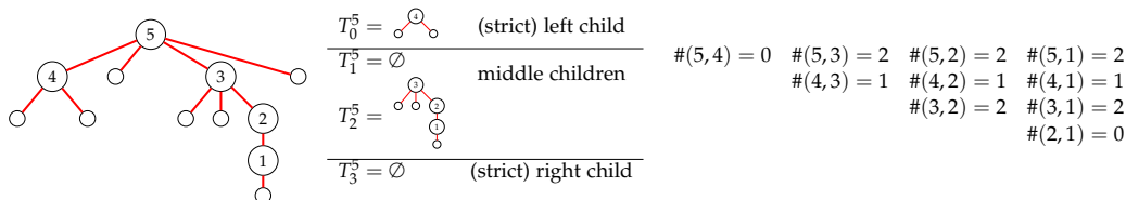
Figure 3: An s -decreasing tree and its tree-inversions for s = (0, 0, 2, 1, 3) .
