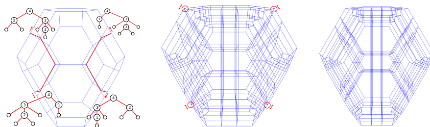
Figure 7: Construction of a 3 dimensional realization.
