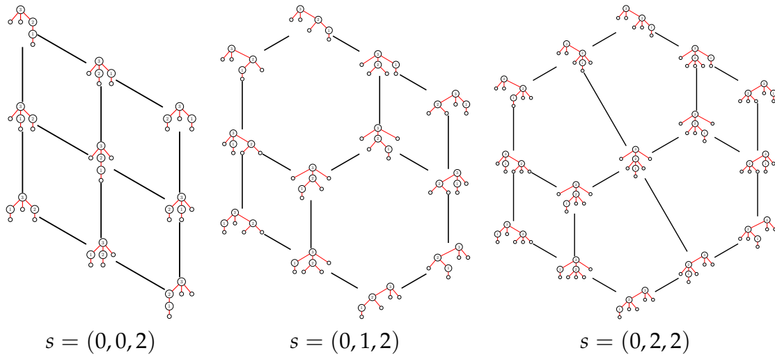
Figure 4: Examples of s -weak lattices.
