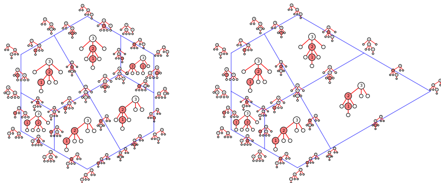
Figure 1: The s -permutahedron and the s -associahedron for s = (0, 2, 2) . Their edge graphs are the Hasse diagrams of the s -weak order and the s -Tamari lattice, respectively.
