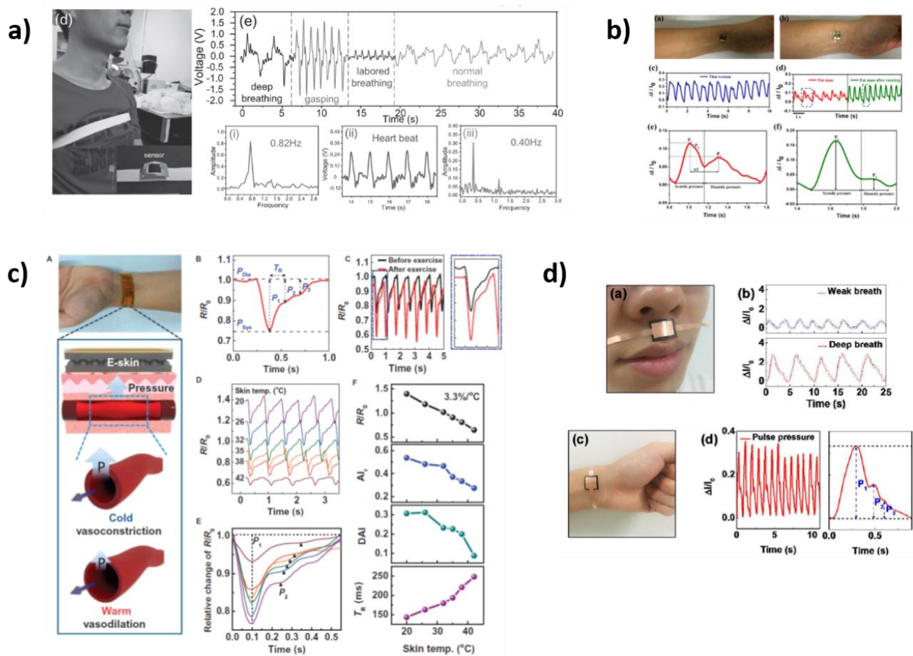
Figure 6. (a) Identification the different breathing modes, labored breathing is additionally enlarged [204] (Reprinted with the permission from Wiley), (b) monitoring of wrist pulse under normal and exercise conditions [205], (c) heart beating and breathing monitoring: simultaneous monitoring of artery pulse and temperature [206], (d) monitored weak and deep breathing and pulse signals [203] (Reprinted with the permission from the American Chemical Society).
