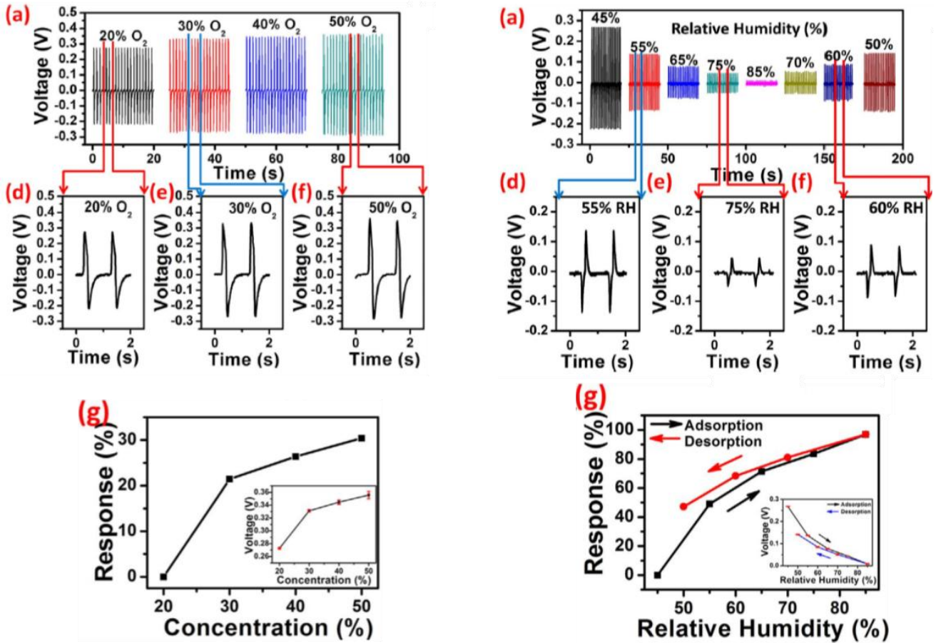
Figure 5. Detection of atmospheric conditions such as O 2 concentration and relative humidity. Reprinted from [201] with the permission from Elsevier.
