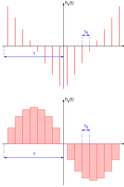
Fig. 2. Convolution kernels of PVAR from phase data (above) or frequency deviations (below) for \tau = 8\tau_0 .
