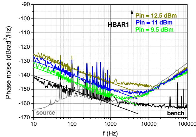
Figure 6: Residual phase noise of the HBAR resonator for various values of the incident microwave power.
