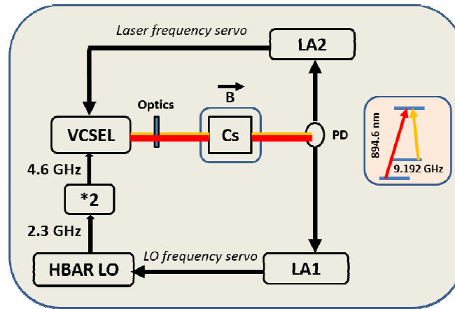
Figure 9: Principle of the CPT atomic clock. The HBAR LO 2.3 GHz signal is frequency doubled to 4.596 GHz. This signal drives a VCSEL laser which generates a bi-chromatic optical field at 895 nm. The laser beam is shaped, circularly polarized and sent into a Cs vapor micro-fabricated cell filled with Ne buffer gas. When the frequency difference between both optical lines is exactly equal to 9.192 GHz, atoms are pumped in a so-called dark state which increases the light transmission through the cell. The CPT resonance is detected by a photodiode. The output signal of the photodiode is sent into two lockin amplifiers (LA). LA1 is used for laser frequency stabilization by synchronously modulating-demodulating the laser dc current (laser frequency). LA2 is used for the HBAR LO frequency by synchronously modulating-demodulating the VCPS in the HBAR oscillator. The output 4.6 GHz at the output of the doubler is extracted with a coupler (not shown on the figure) and compared to the 4.6 GHz signal from a high-performance commercial microwave synthesizer driven by a hydrogen maser for frequency stability measurement. The inset on the right of the figure shows the energy diagram involved in the CPT phenomenon.
