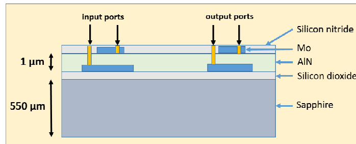
Figure 1: Architecture of the AlN-Sapphire HBAR resonator.
