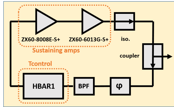
Figure 7: Architecture of the HBAR-based 2.3 GHz oscillator
