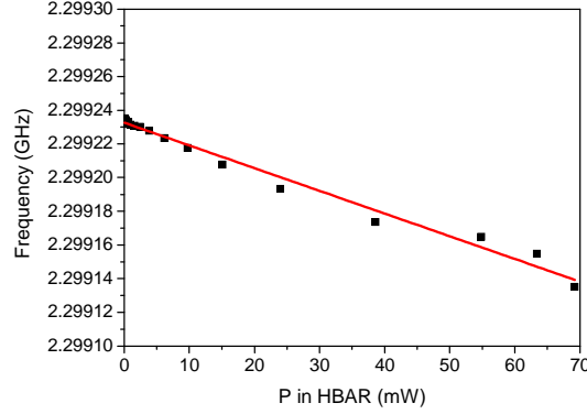
Figure 5: Frequency of the HBAR resonance versus the input port microwave power.
