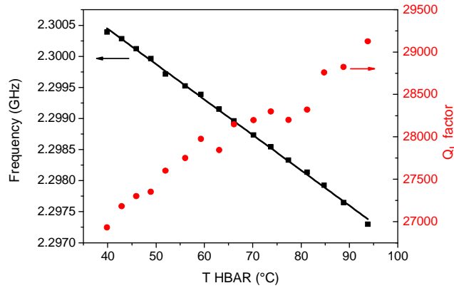
Figure 4: Frequency and Q_L factor of the HBAR versus the temperature.
