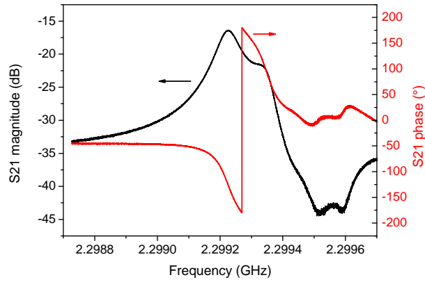
Figure 3: S_{21} parameter (magnitude and phase) of the HBAR resonator mode at about 2.3 GHz.
