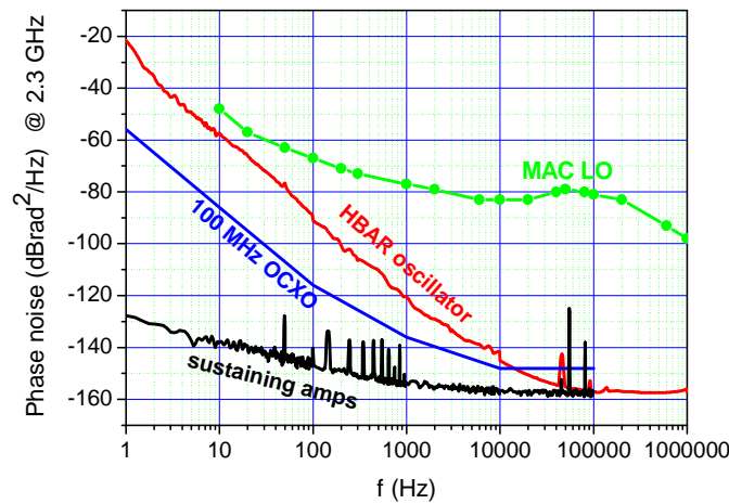
Figure 8: Phase noise of the sustaining amplifier and HBAR-based oscillator at 2.3 GHz. The latter is compared with the absolute phase noise of a state-of-the-art 100 \text{ MHz} OCXO ideally frequency-multiplied to 2.3 \text{ GHz} . Also, the phase noise at 2.3 \text{ GHz} of a conventional MAC LO [12] is reported for comparison.
