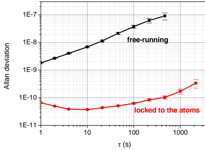
Figure 10: Allan deviation of the HBAR oscillator in free-running and locked regime (to the atoms).
