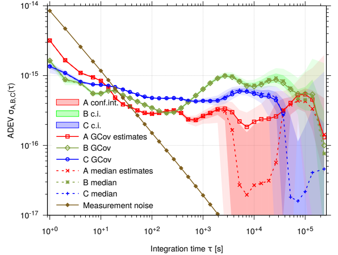
Fig. 5. GCov measurements of a set of 3 Cryogenic Sapphire Oscillators of FEMTO-ST. The confidence intervals are represented by colored areas: bright colors for 68 % c.i. ( 1 \sigma ) and pale colors for 95 % c.i. ( 2 \sigma ). The brown line shows the measurement noise obtained from the closure. The linear frequency drifts of the CSO have been removed.
