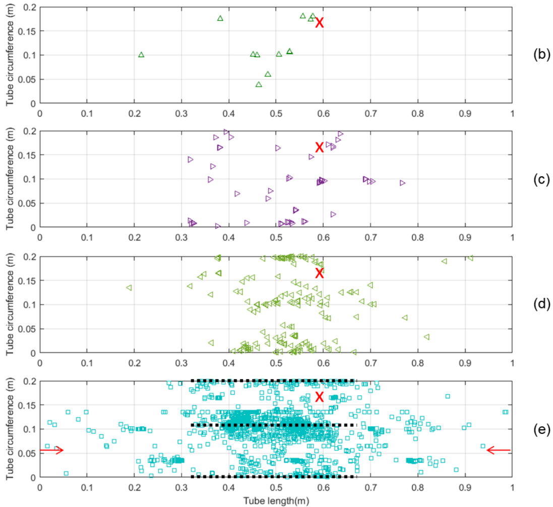
Figure 4. Estimated damage locations during loading of specimen 1: (a) cycle 1 (blue v), (b) cycle 2 (green \wedge ), (c) cycle 3 (purple \triangleright ), (d) cycle 4 (lime green \triangleleft ), (e) cycle 5 (turquoise \square ). Dashed lines indicate locations of the through-thickness final failure cracks. Red arrows indicate the top of the specimen.
