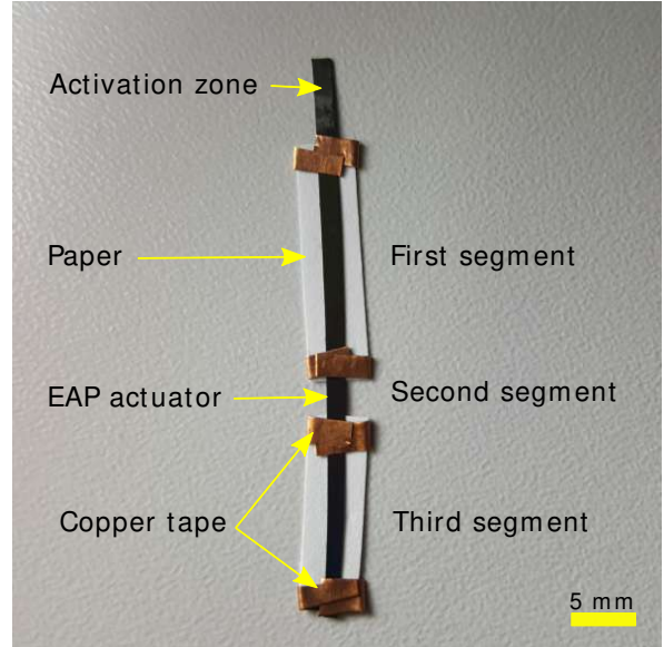
FIGURE 4. Top view of the three-segment self-folding straight structure.
