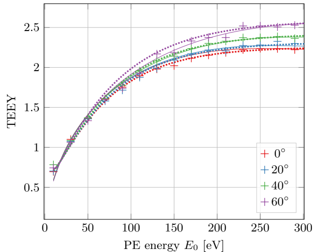
FIG. 6: Measured and fitted TEEY on Cu #2 (as received; + measures, ..... Dionne fit, — Vaughan fit).
